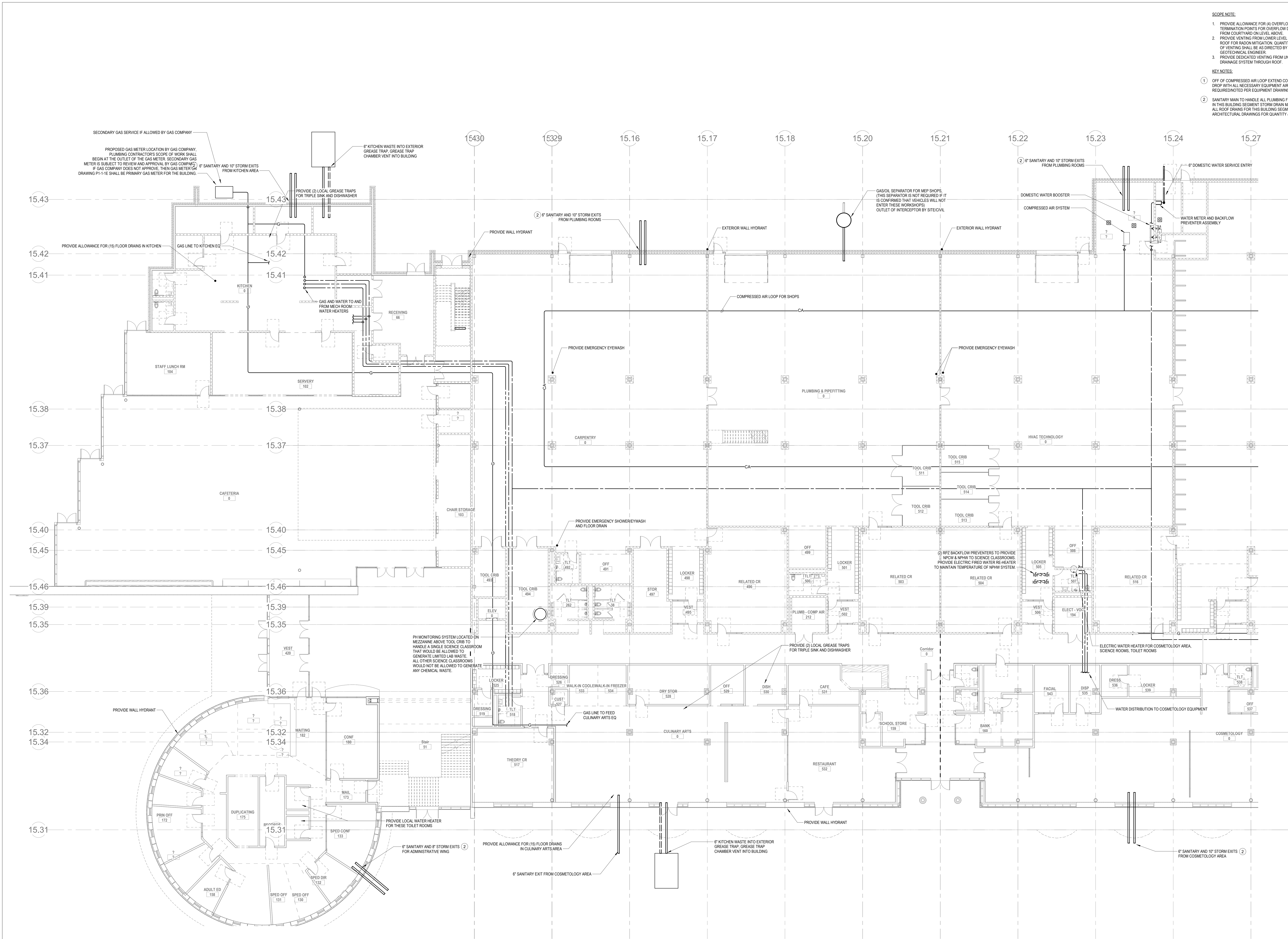
2 PLUMBING Level 1 West 3/32" = 1'-0"
