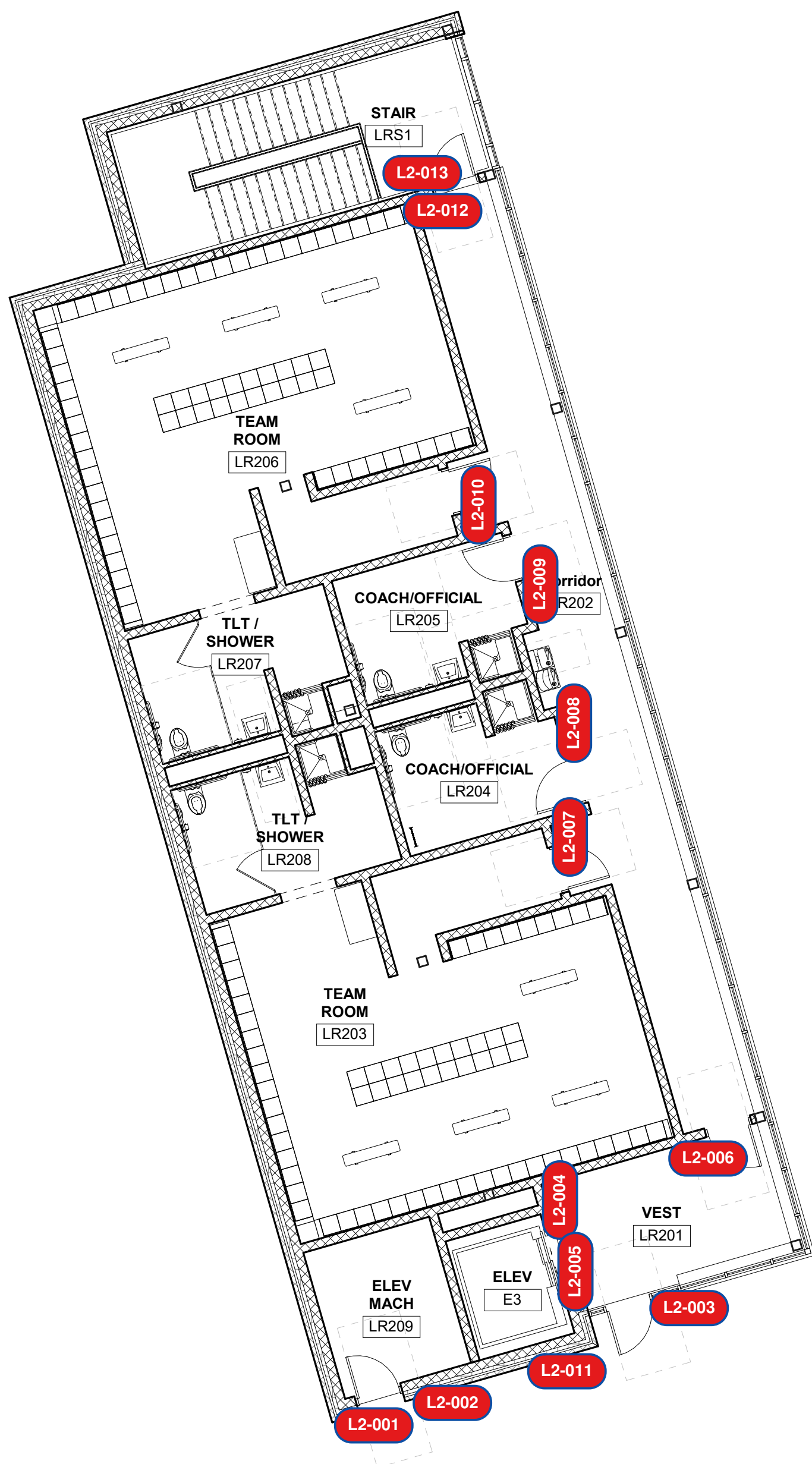
1 LOCKER BUILDING SECOND FLOOR SIGNAGE PLAN 1/8" = 1'-0"
