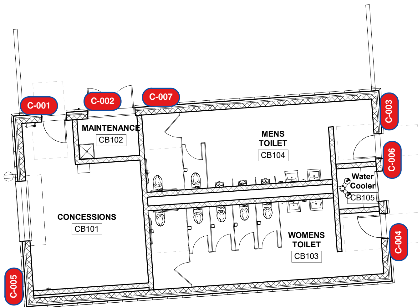
1 CONCESSION BUILDING SIGNAGE PLAN 1/8" = 1'-0"
