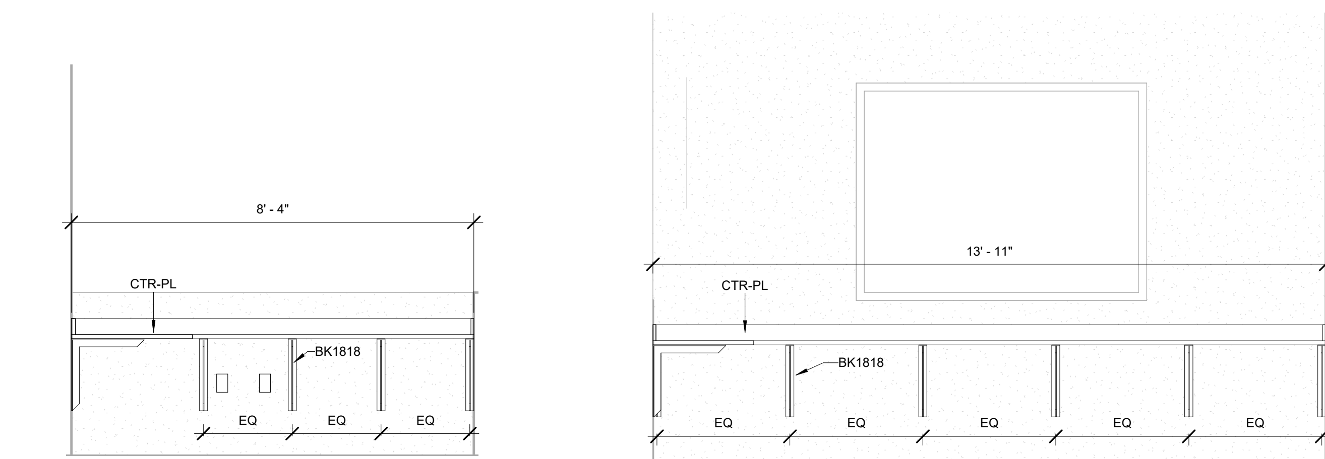
11 B301D - Health Assist - Office - North 1/2" = 1'-0"
