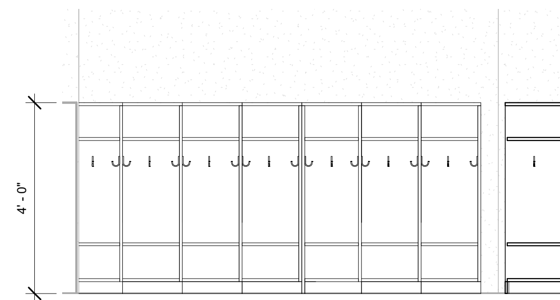
15 C106A - CUBBIES, East 1/2" = 1'-0"
