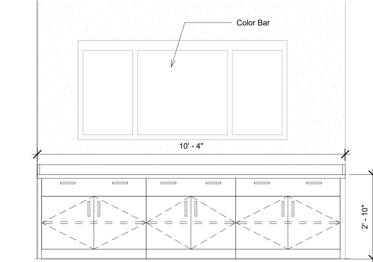
11 B120B - Cosmetology - Dispensary - South 1/2" = 1'-0"
