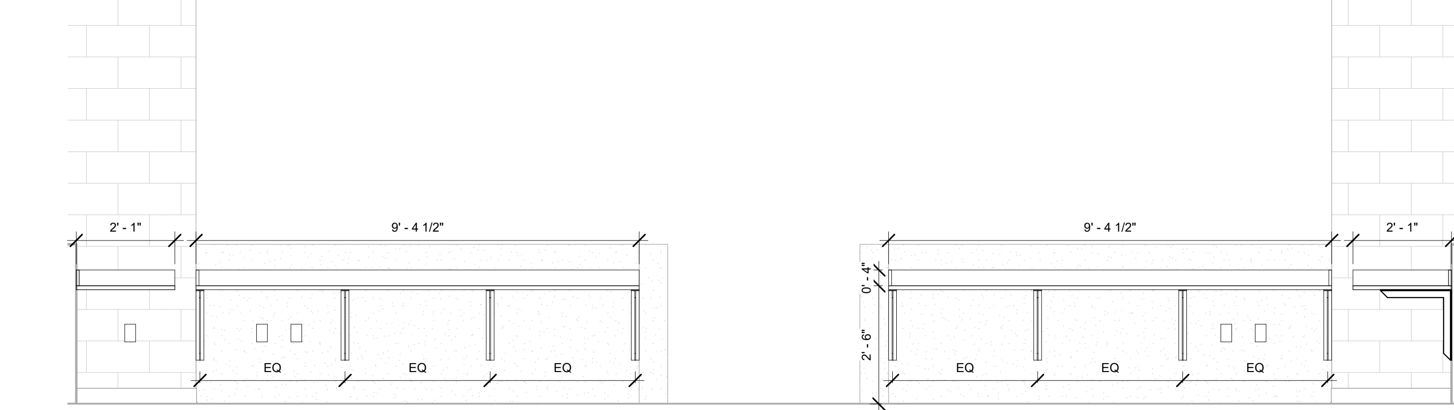
6 B104 - Electrical - Staff Office - North 1/2" = 1'-0"
