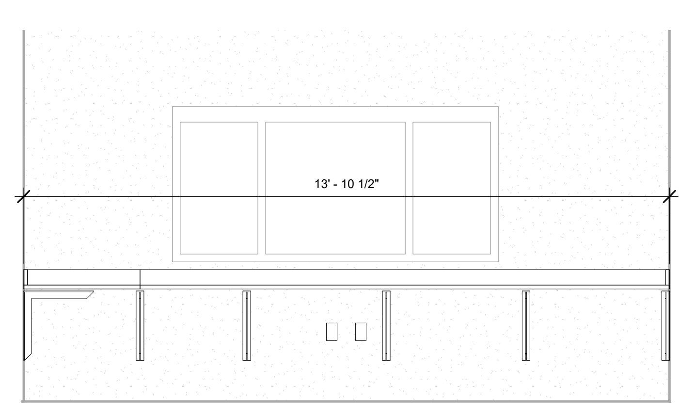
8 B121C- Office-South 1/2" = 1'-0"
