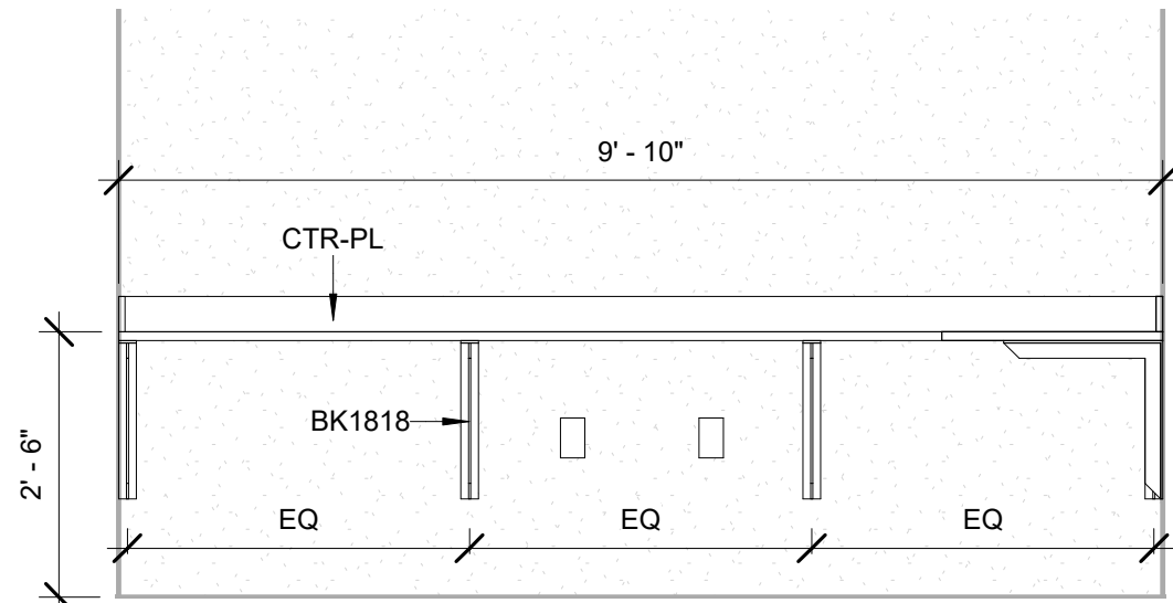
2 B202D - Business Tech- Office - South 1/2" = 1'-0"
