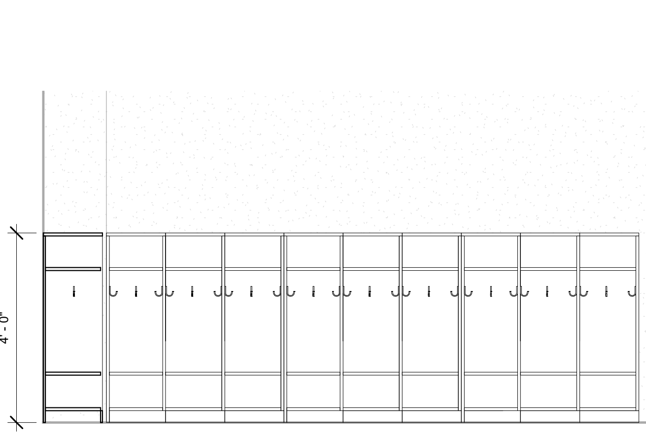
17 C106A - CUBBIES, South 1/2" = 1'-0"
