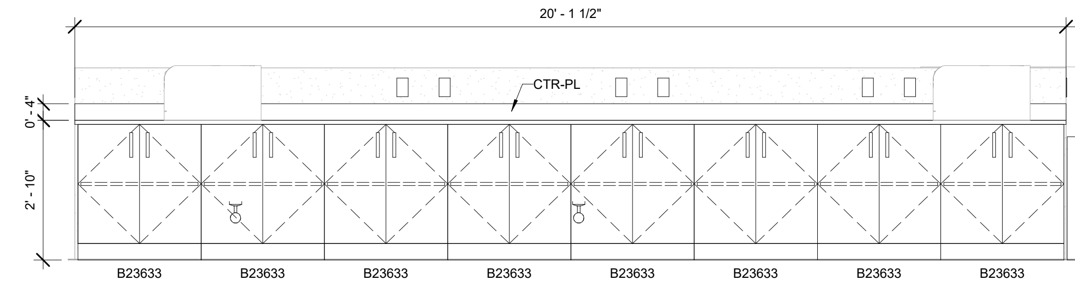
③ A206 - Design Visual Comm, East 1/2" = 1'-0"
