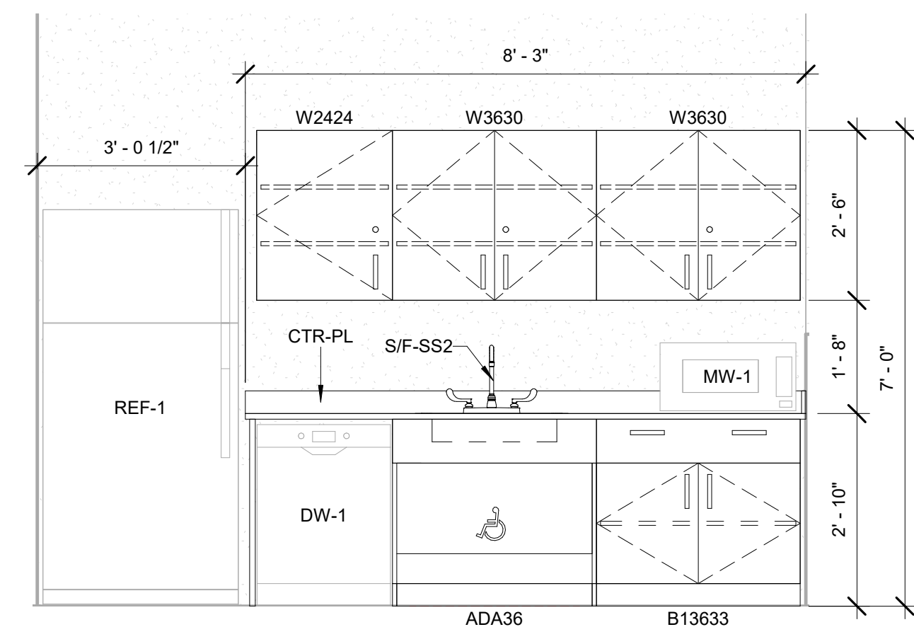
18 C106J - Kitchen, North 1/2" = 1'-0"
