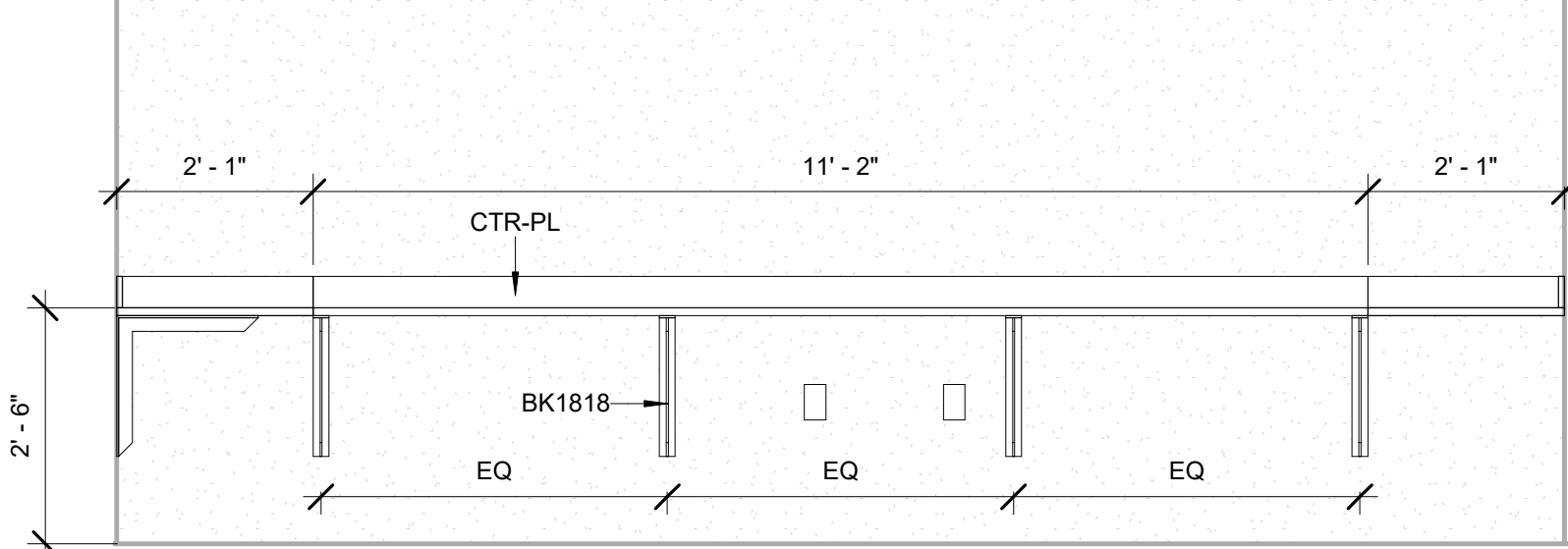
3 B202D - Business Tech- Office- West 1/2" = 1'-0"
