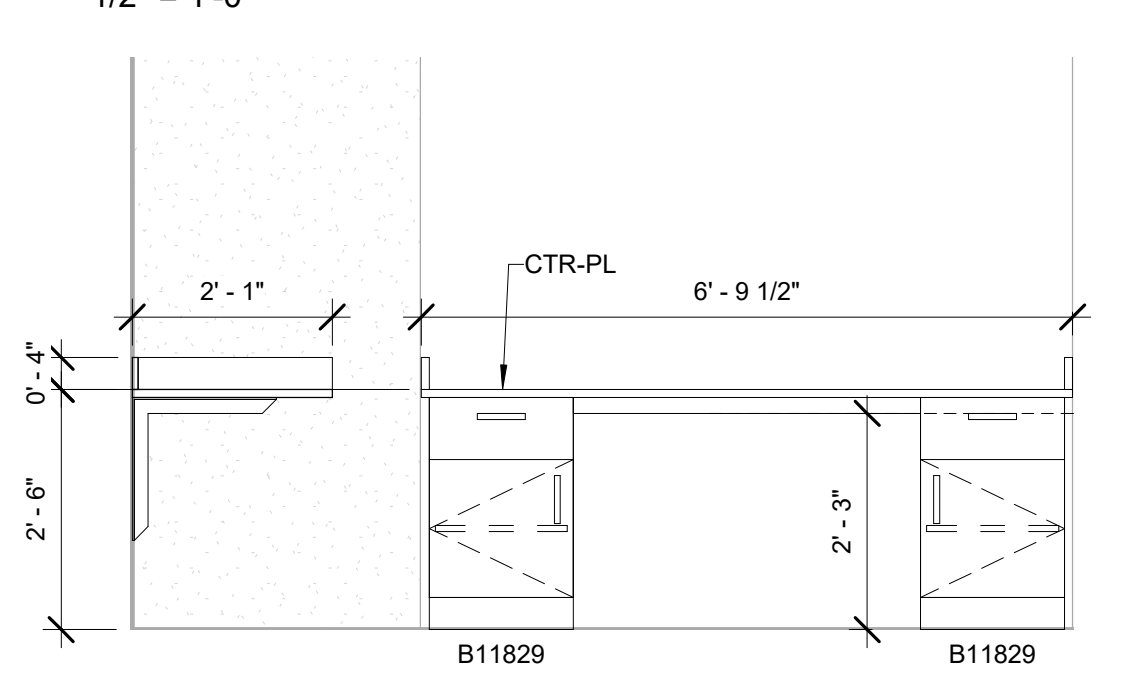
⑭ A206G - Design Visual Comm- Office, West 1/2" = 1'-0"
