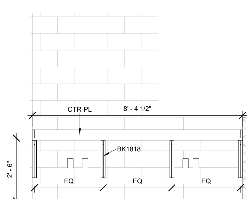
③ Metal Fab - Staff Office - East 1/2" = 1'-0"
