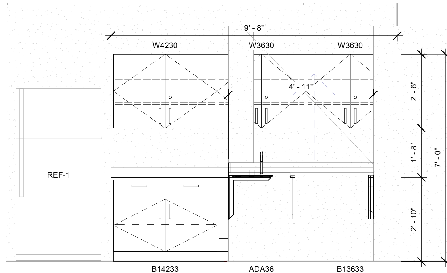
7 B234 - Teacher Plan, West 1/2" = 1'-0"
