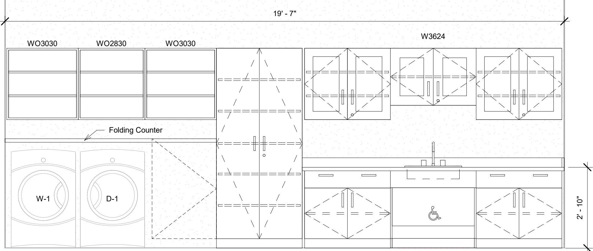
10 B120B - Cosmetology - Dispensary - North 1/2" = 1'-0"
