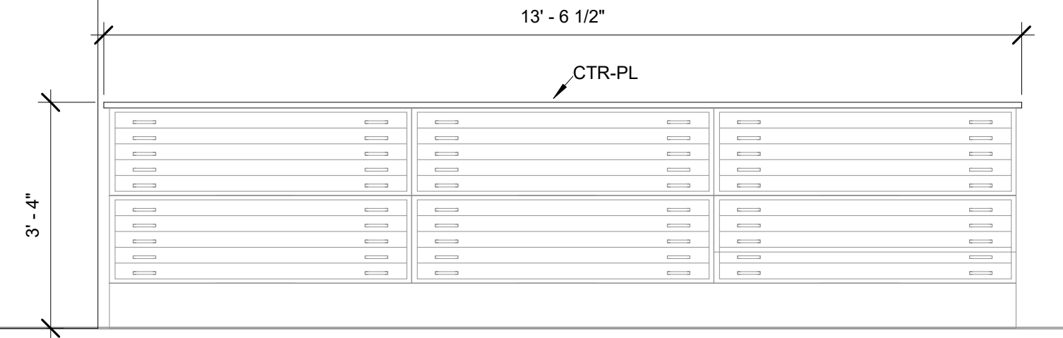
④ A206 - Design Visual Comm, Flat File Counter 1/2" = 1'-0"
