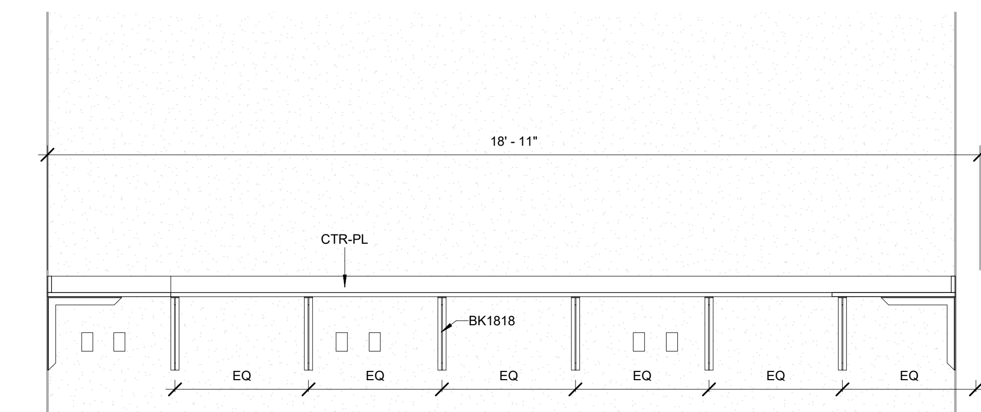
9 B301D - Health Assist - Office - South 1/2" = 1'-0"
