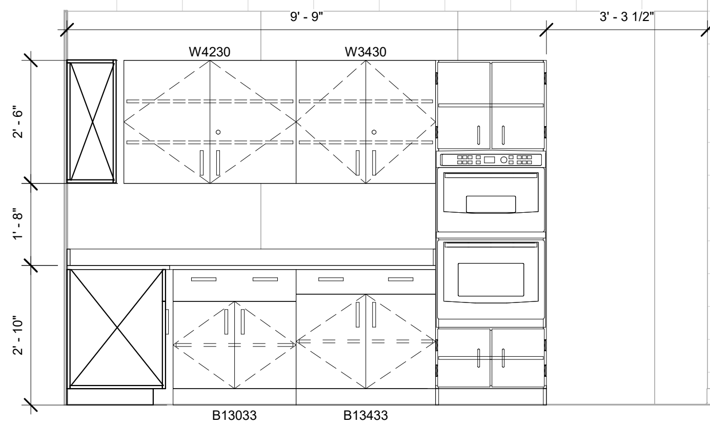
1 B104 - Electrical - Mock Kitchen - North 1/2" = 1'-0"
