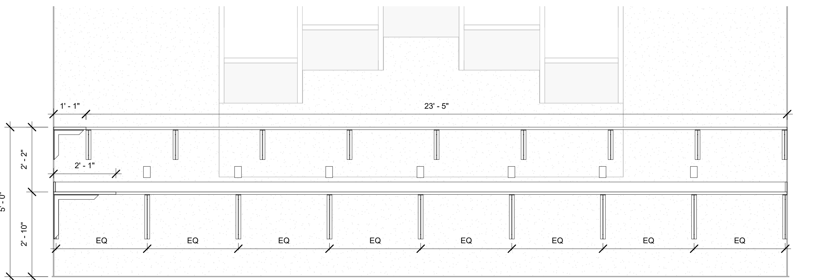
17 B121E- Theory CR-South 1/2" = 1'-0"
