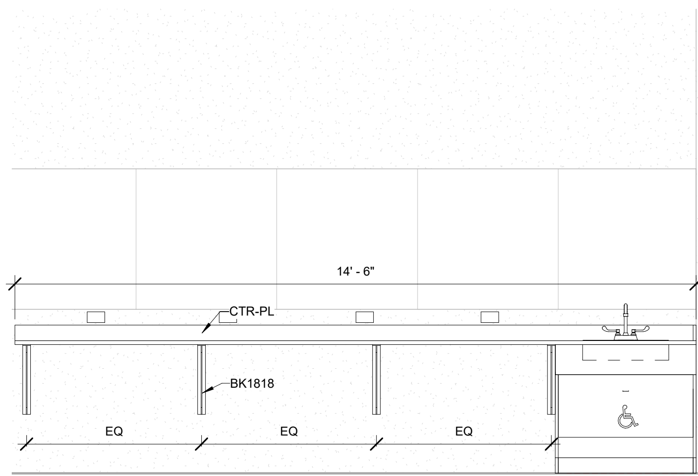
21 C110 - Dressing, North 1/2" = 1'-0"
