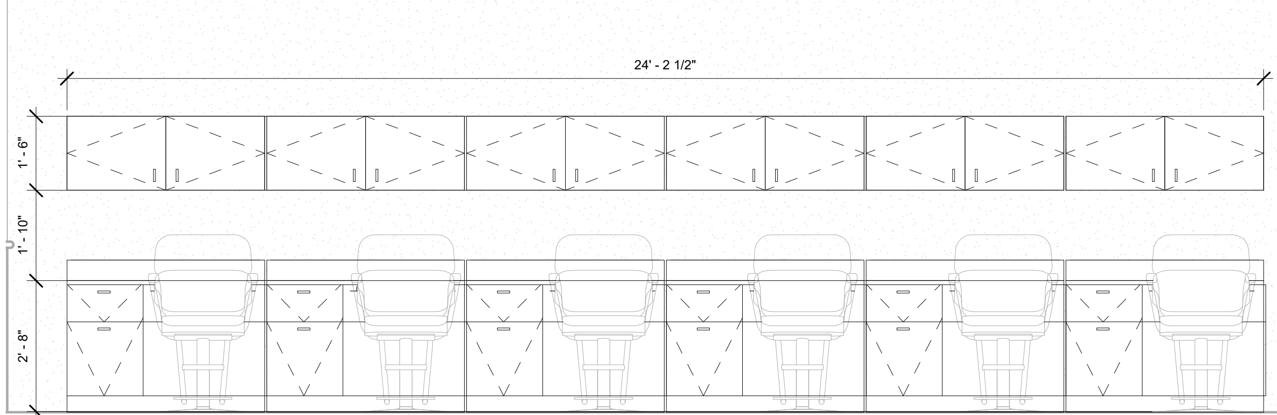
1 B121- Cosmetology- West 1/2" = 1'-0"
