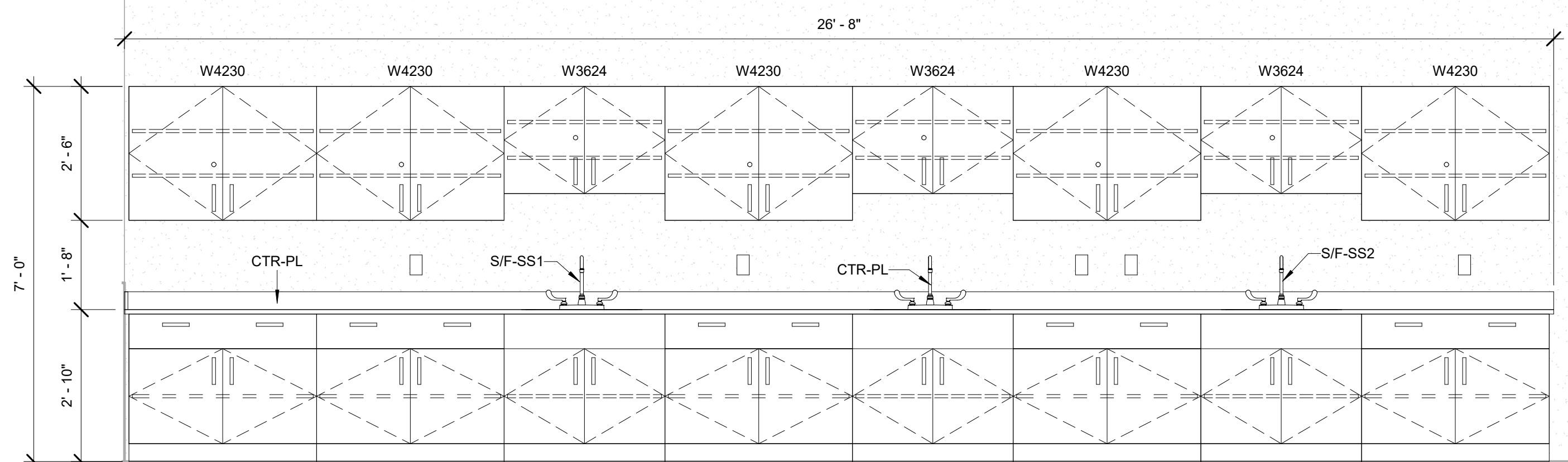
4 A402 - Dental Assist, East 1/2" = 1'-0"
