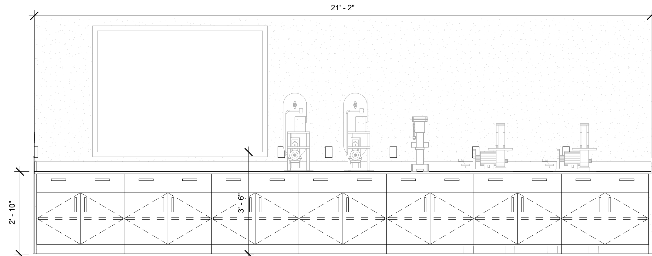
3 B368- Fabrication Lab- East 1/2" = 1'-0"
