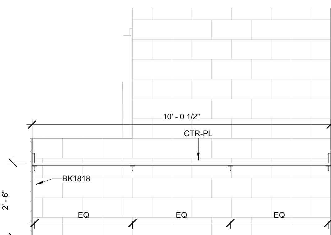
② Metal Fab - Staff Office - West 1/2" = 1'-0"
