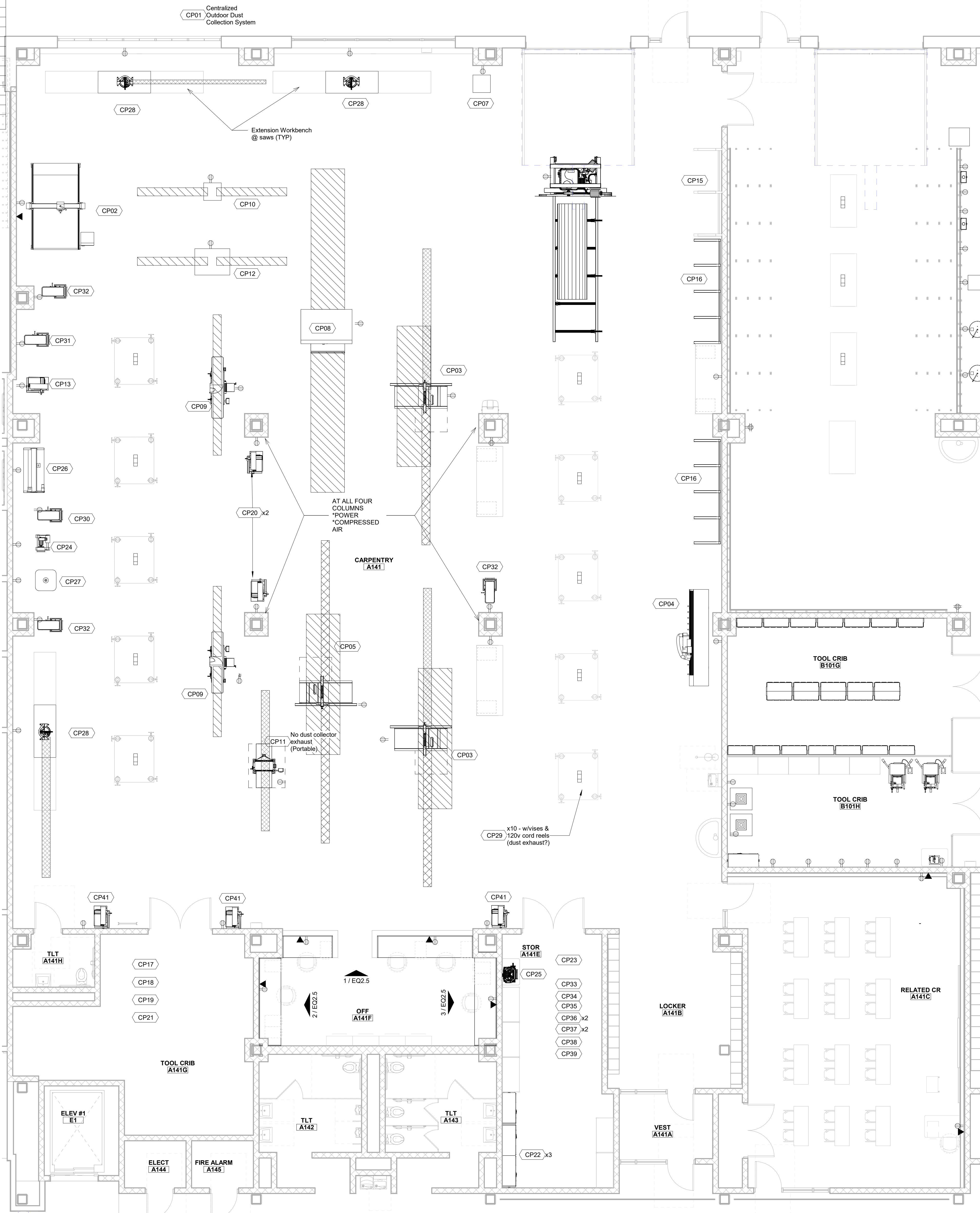
4 Level 1 - Carpentry 3/16" = 1'-0"
