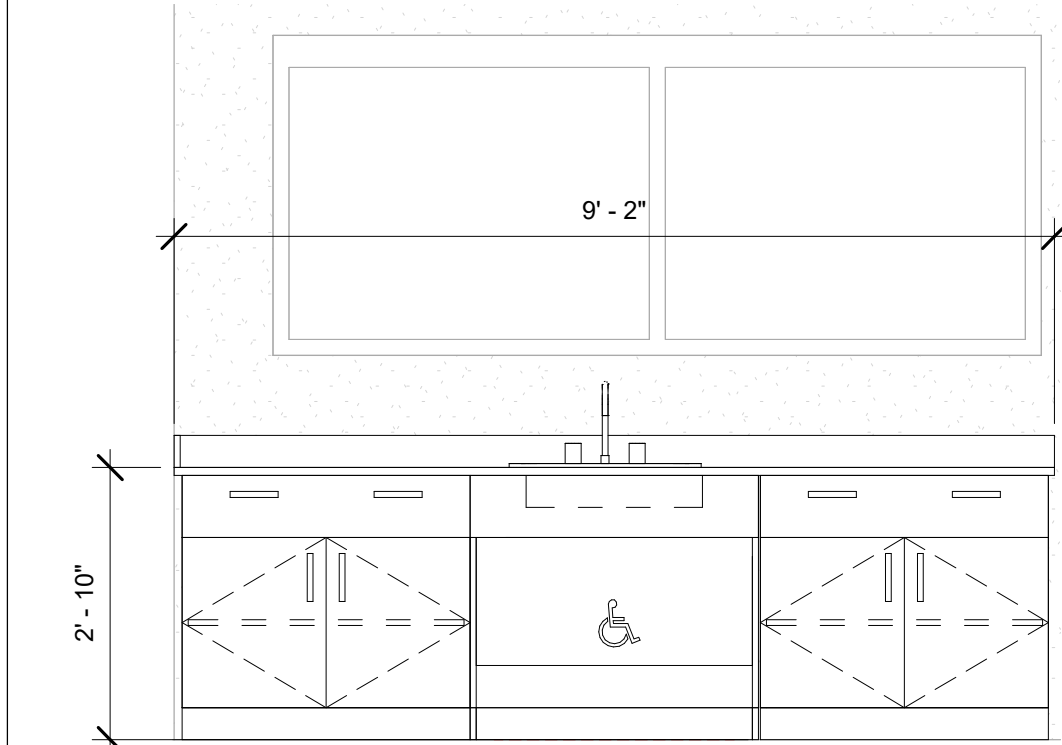
1 B202 - Business Tech Kitchen, North 1/2" = 1'-0"
