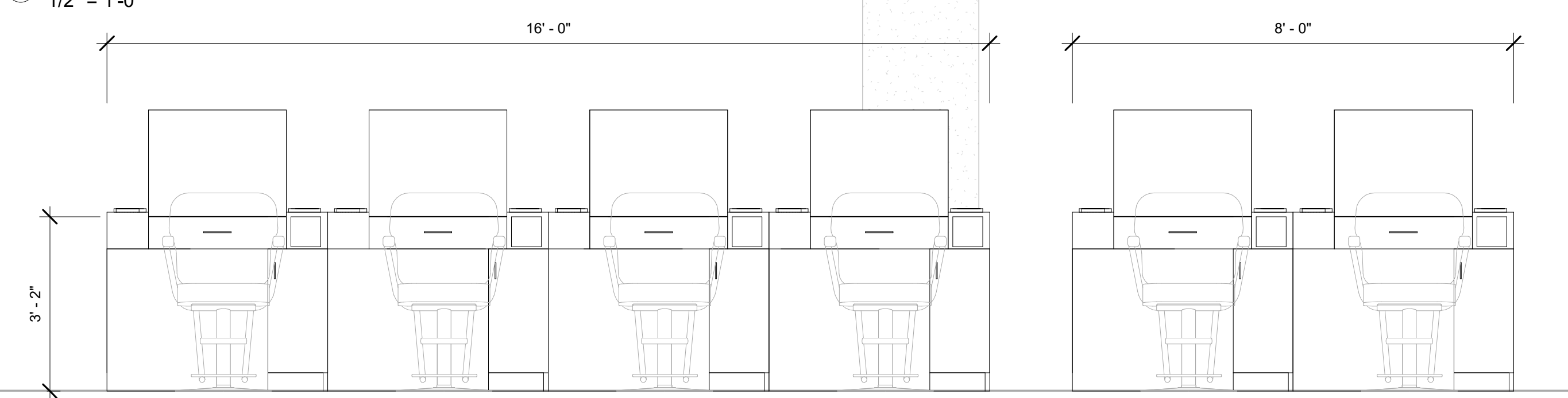
3 B120 - Cosmetology-South 1/2" = 1'-0"
