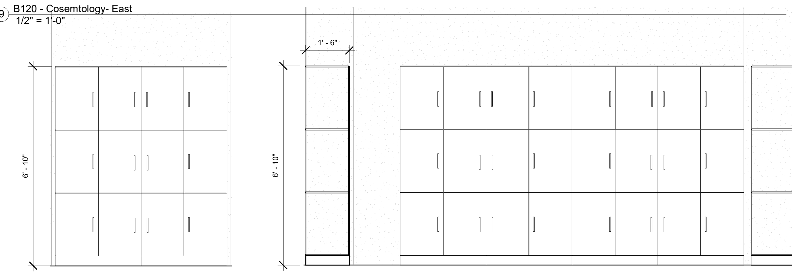
13 B121A - Locker, East 1/2" = 1'-0"
