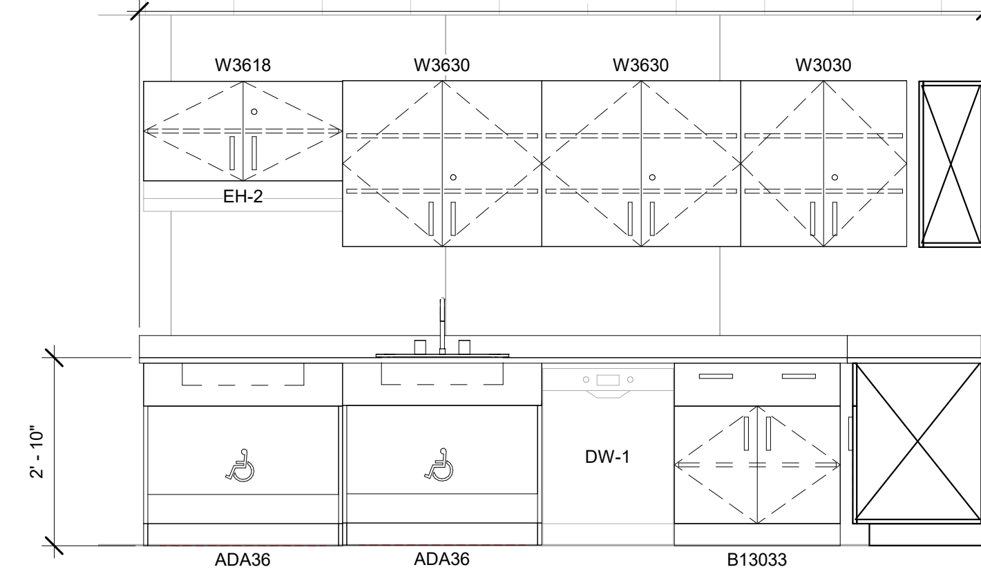
2 B104 - Electrical - Mock Kitchen - West 1/2" = 1'-0"
