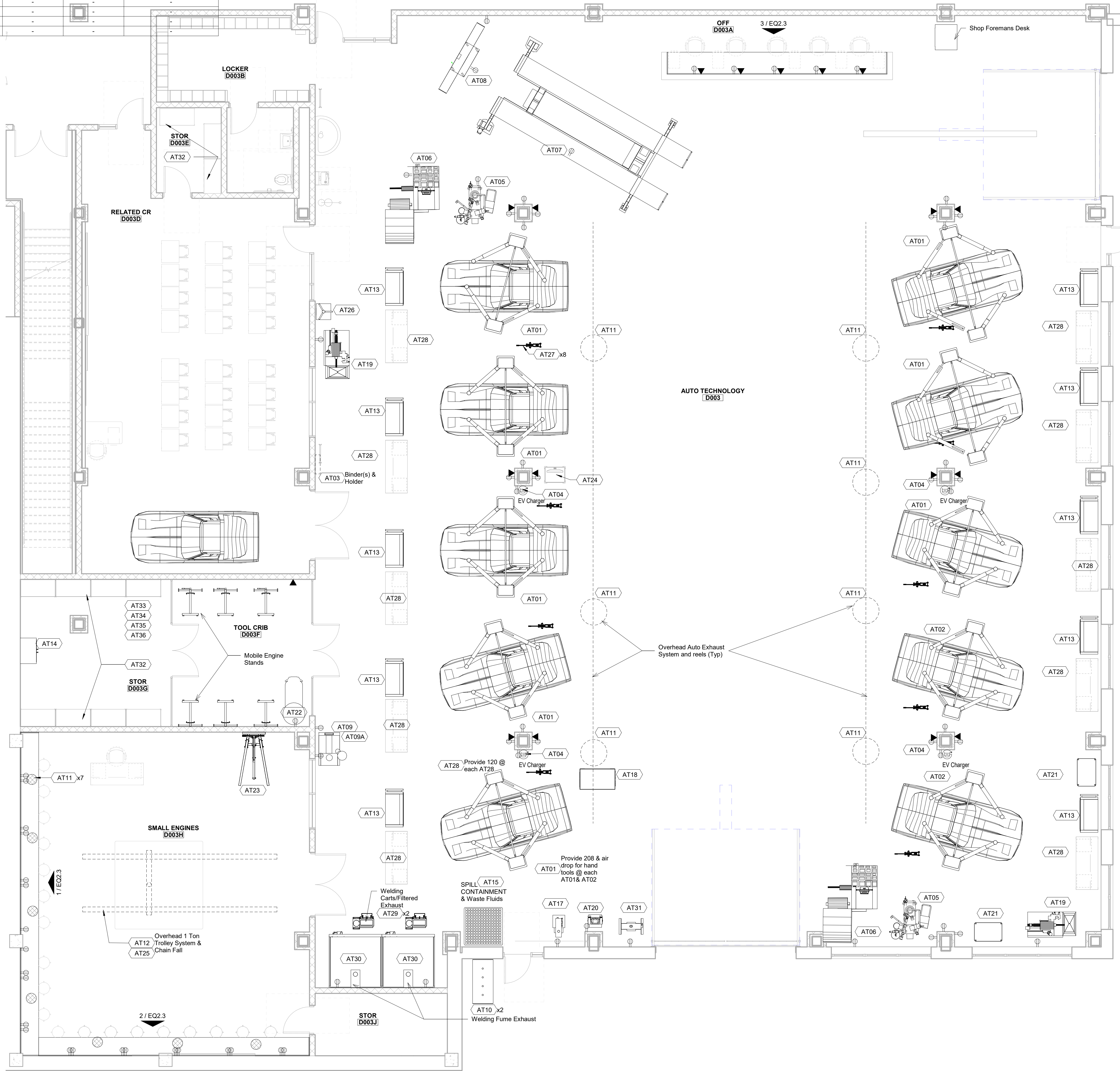
4 Level 0 - Auto Tech 3/16" = 1'-0"
