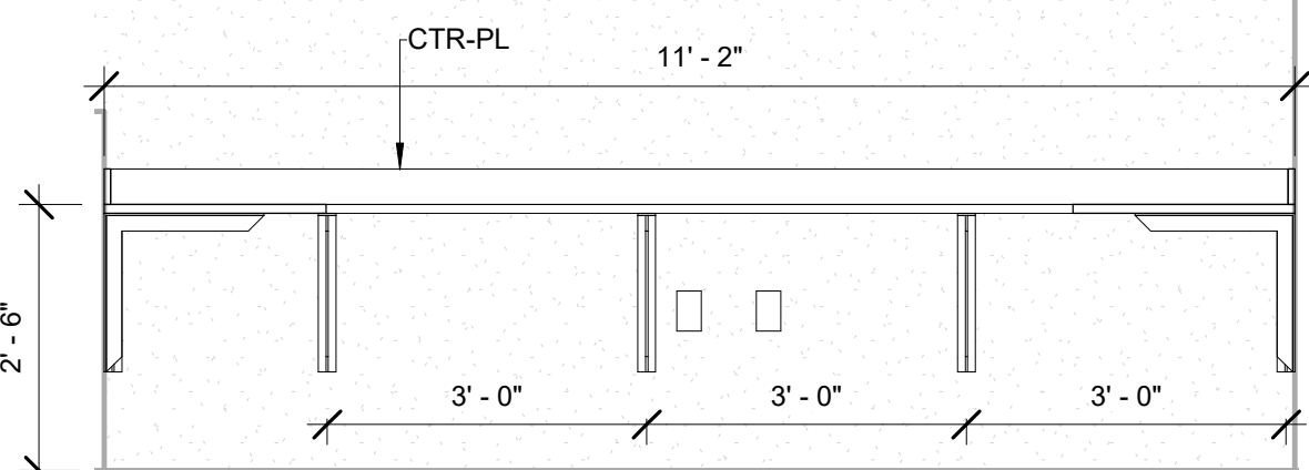
⑫ A206G - Design Visual Comm- Office, East 1/2" = 1'-0"
