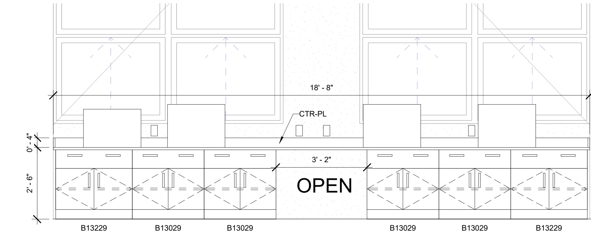
② A206 - Design- Visual Comm, North 1/2" = 1'-0"
