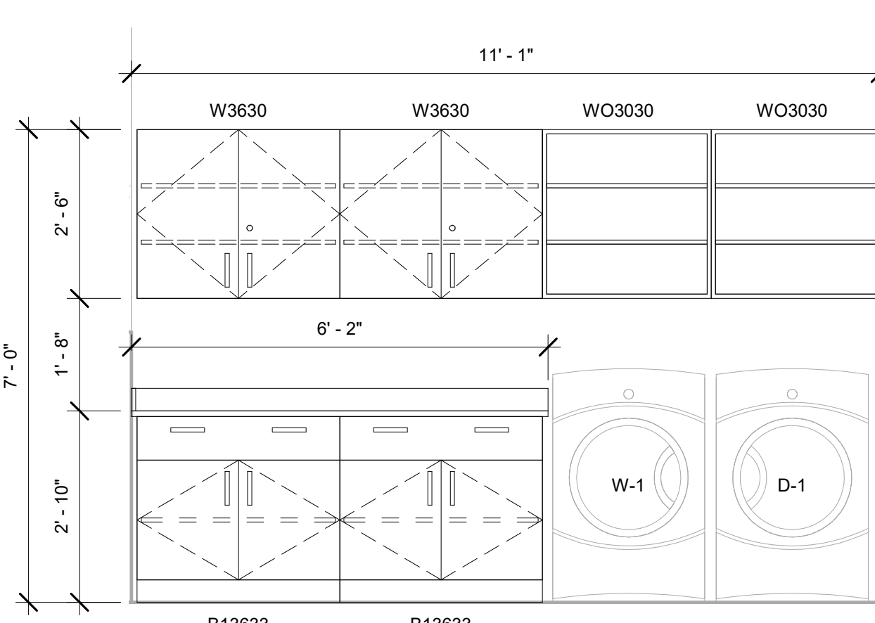
19 C106J - Kitchen, South 1/2" = 1'-0"
