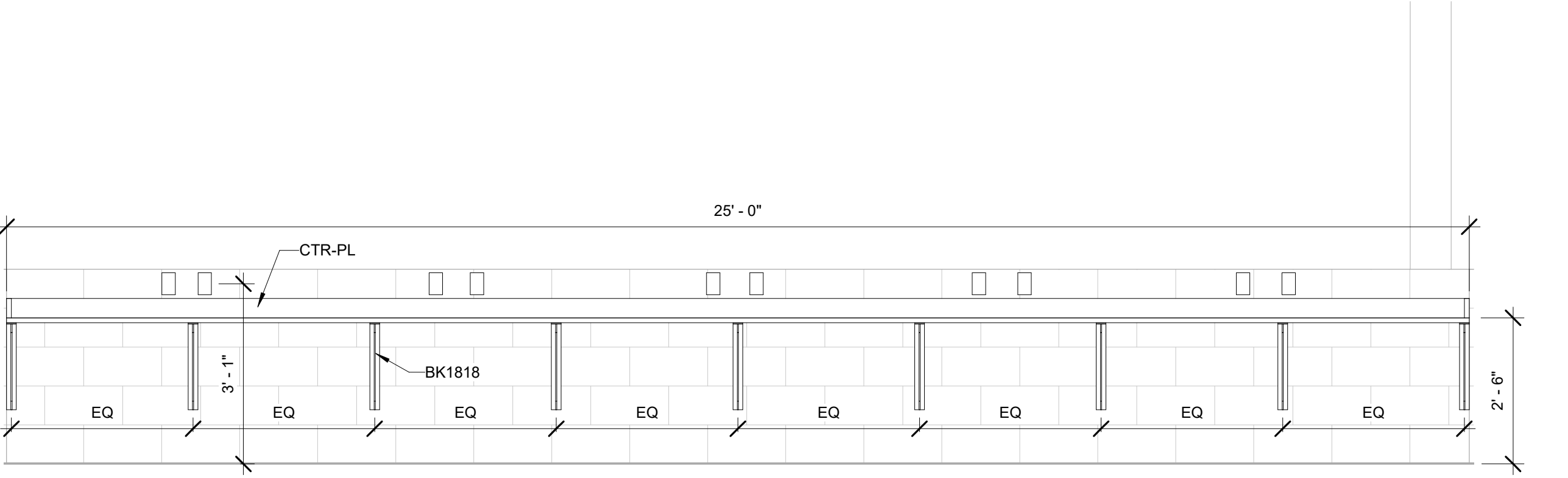
3 Auto Tech Staff Office 1/2" = 1'-0"
