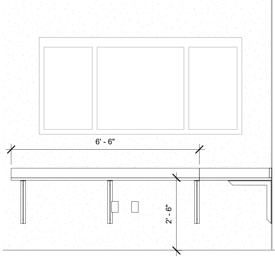
5 B120A - Cosmetology - Staff Office - South 1/2" = 1'-0"
