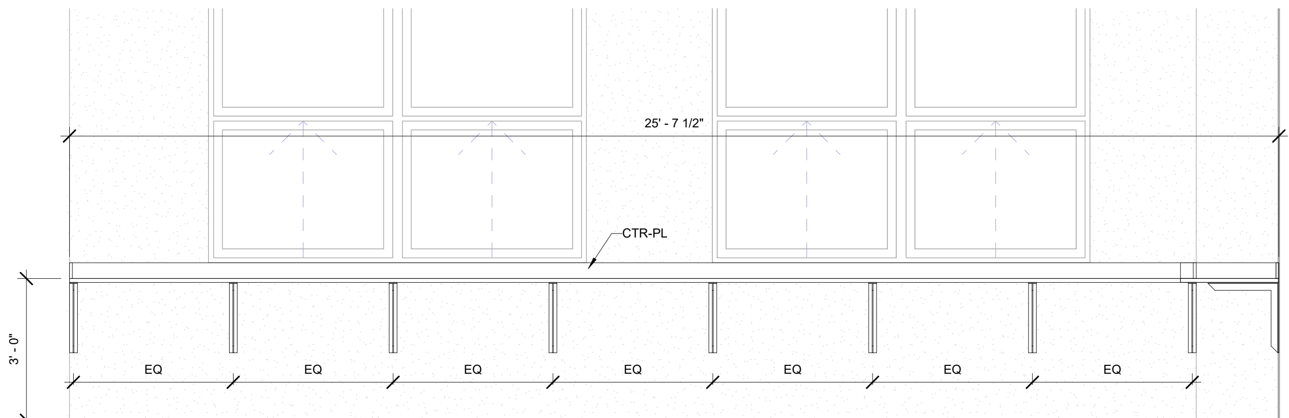
12 B203C - Computer Lab, North 1/2" = 1'-0"
