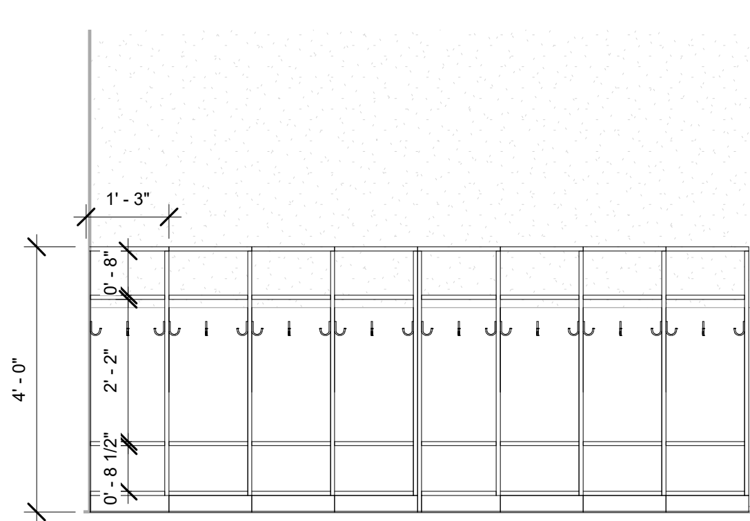
16 C106A - CUBBIES, North 1/2" = 1'-0"
