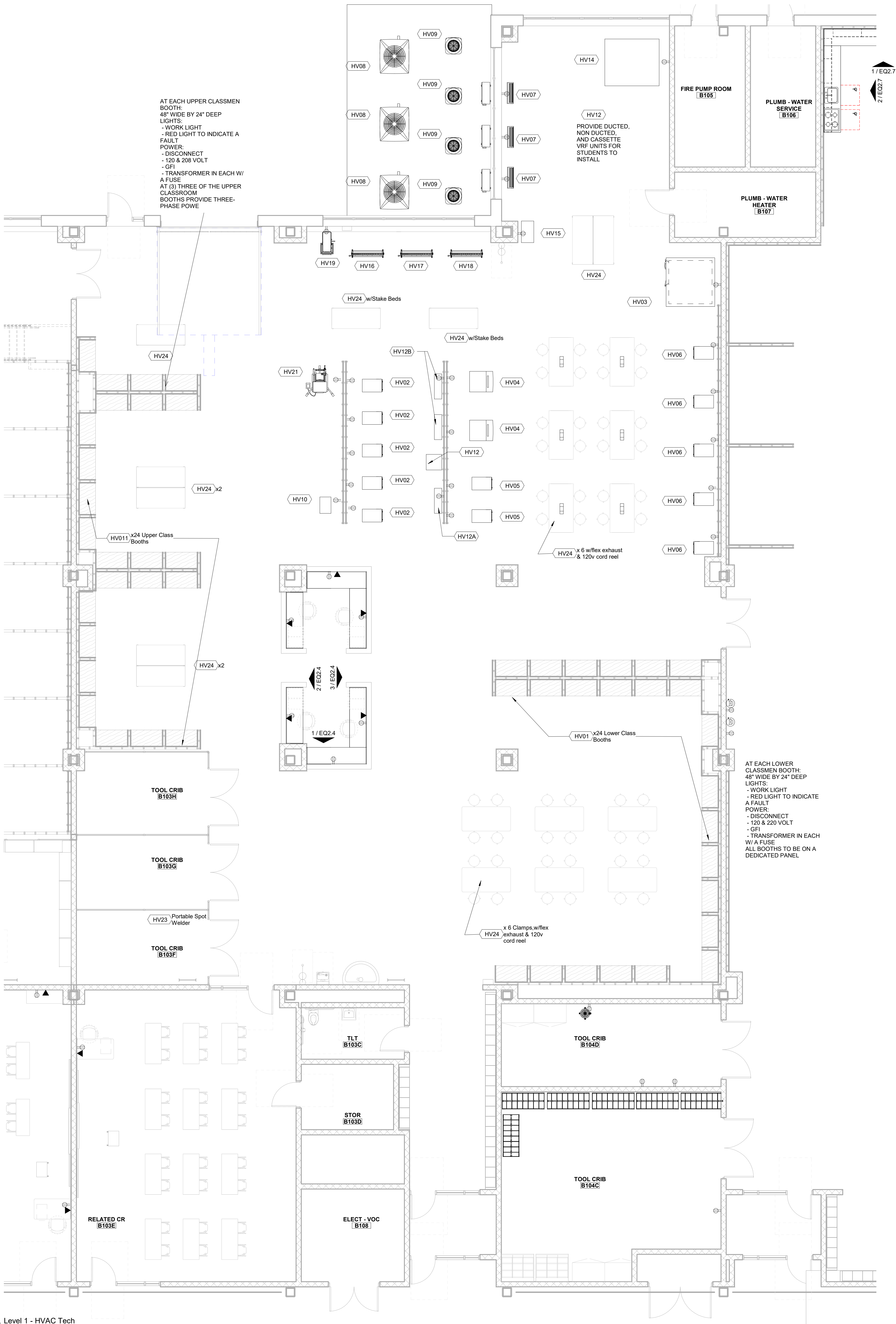
5 Level 1 - HVAC Tech 3/16" = 1'-0"
