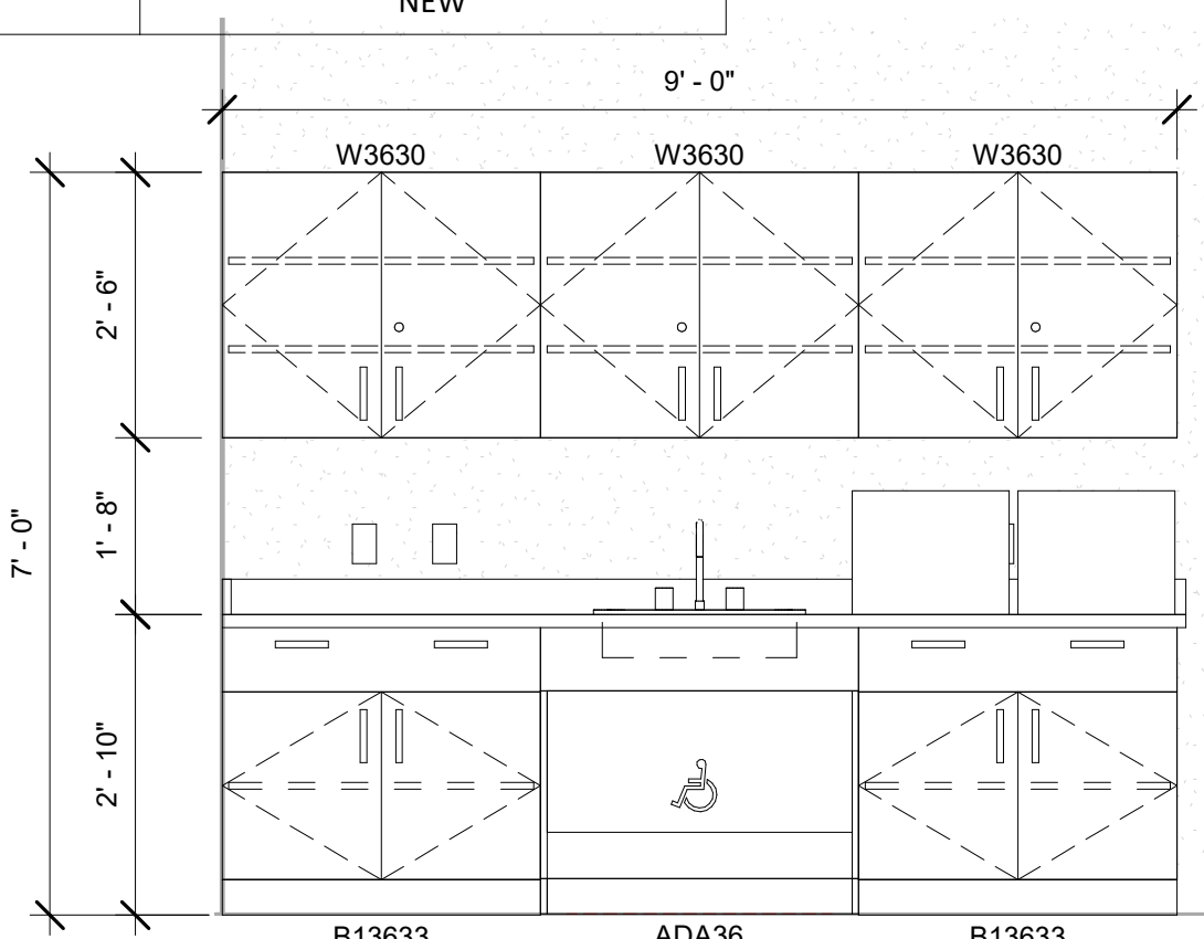
4 B120C - Cosmetology - Facial 1/2" = 1'-0"
