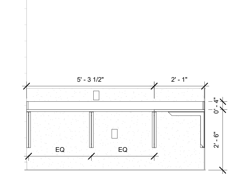
3 B104 - Electrical - Staff Office - East 1/2" = 1'-0"
