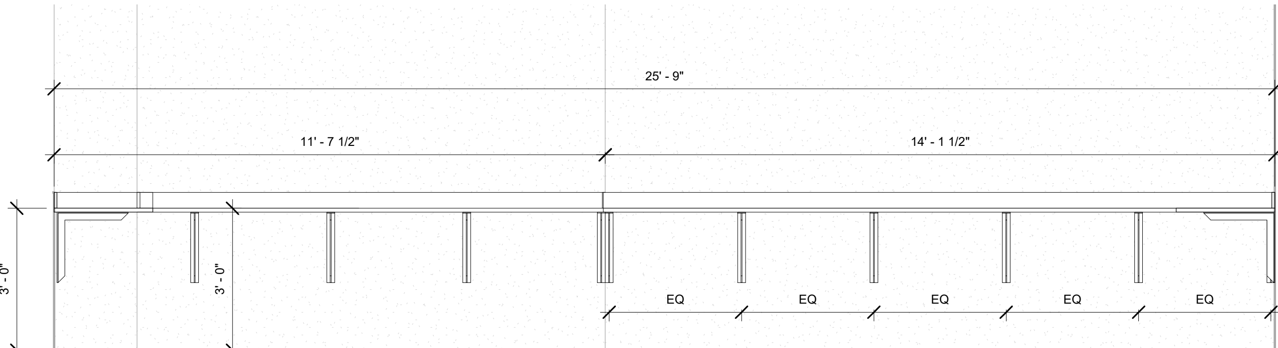
11 B203C - Computer Lab, East 1/2" = 1'-0"
