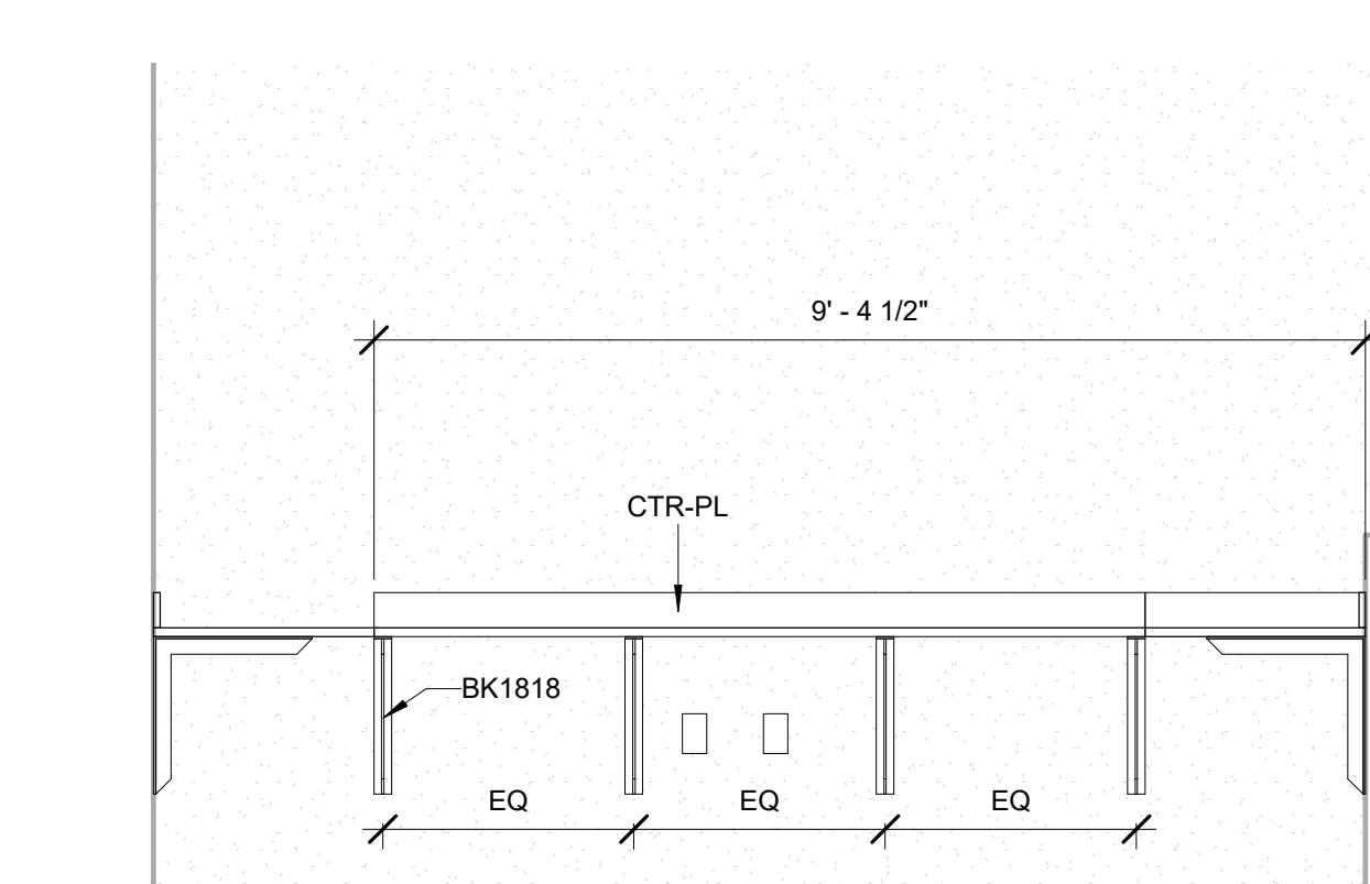
10 B301D - Health Assist - Office - West 1/2" = 1'-0"
