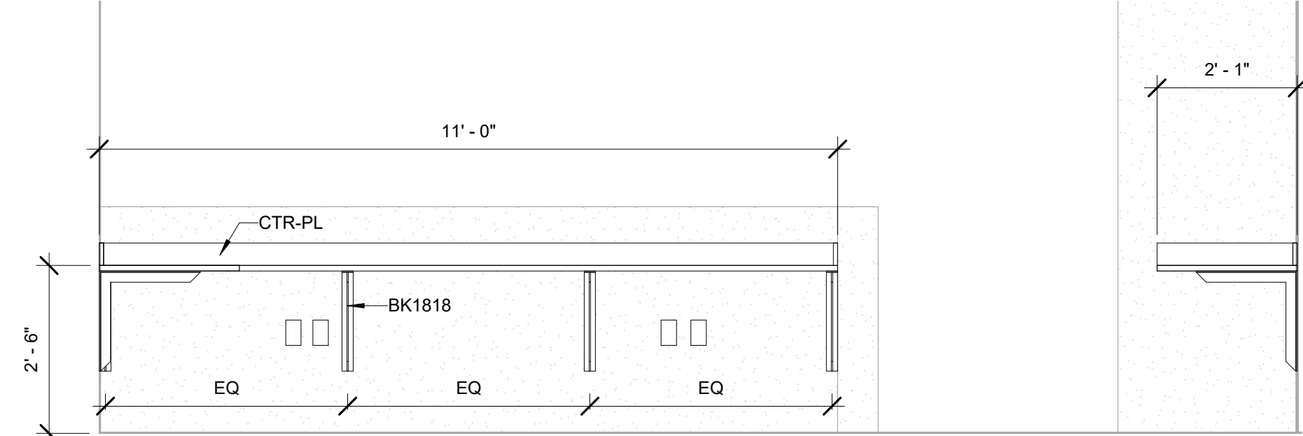
8 A402G - Dental Assist- Office, North 1/2" = 1'-0"
