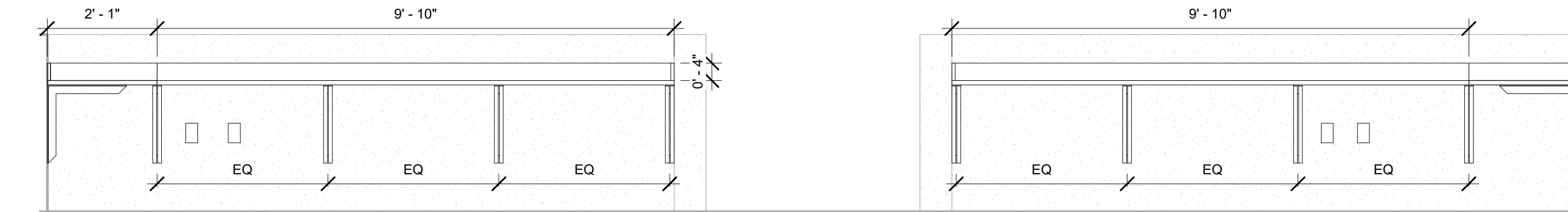
5 B104 - Electrical - Staff Office - South 1/2" = 1'-0"
