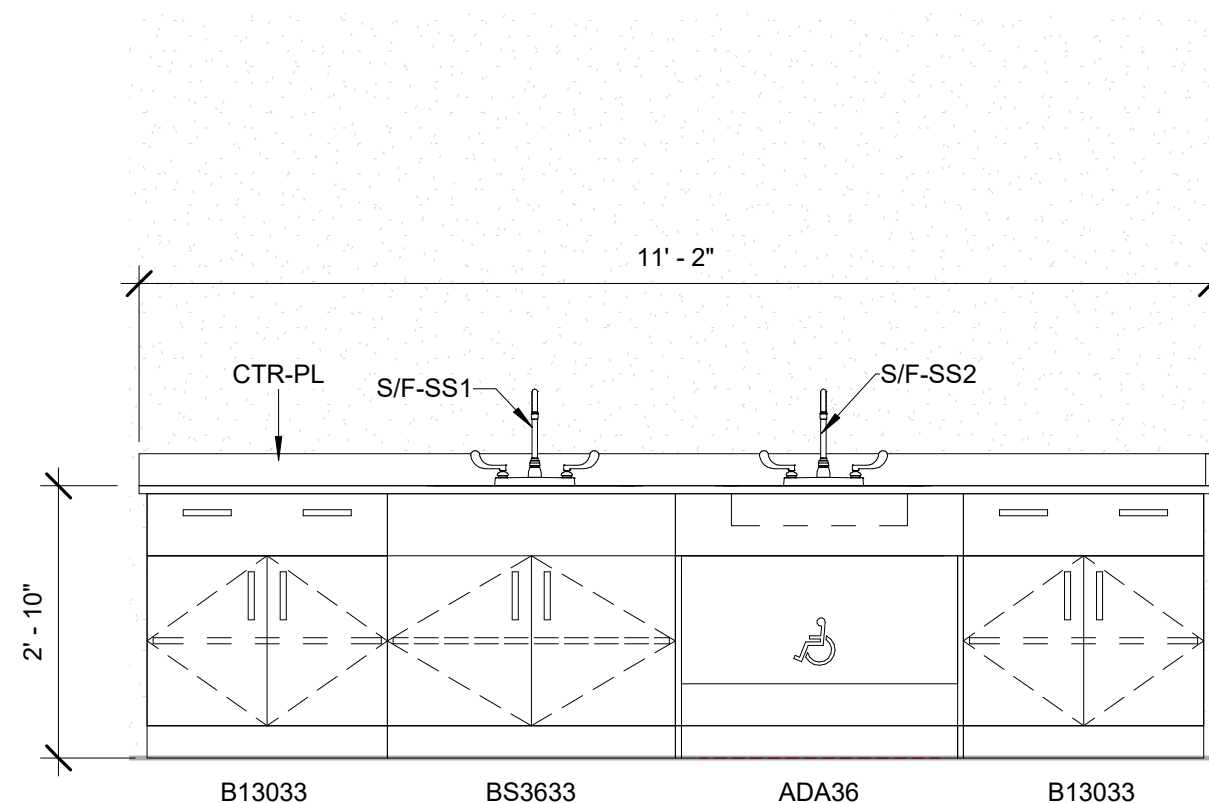
14 C106 - Early Childhood, West 1/2" = 1'-0"
