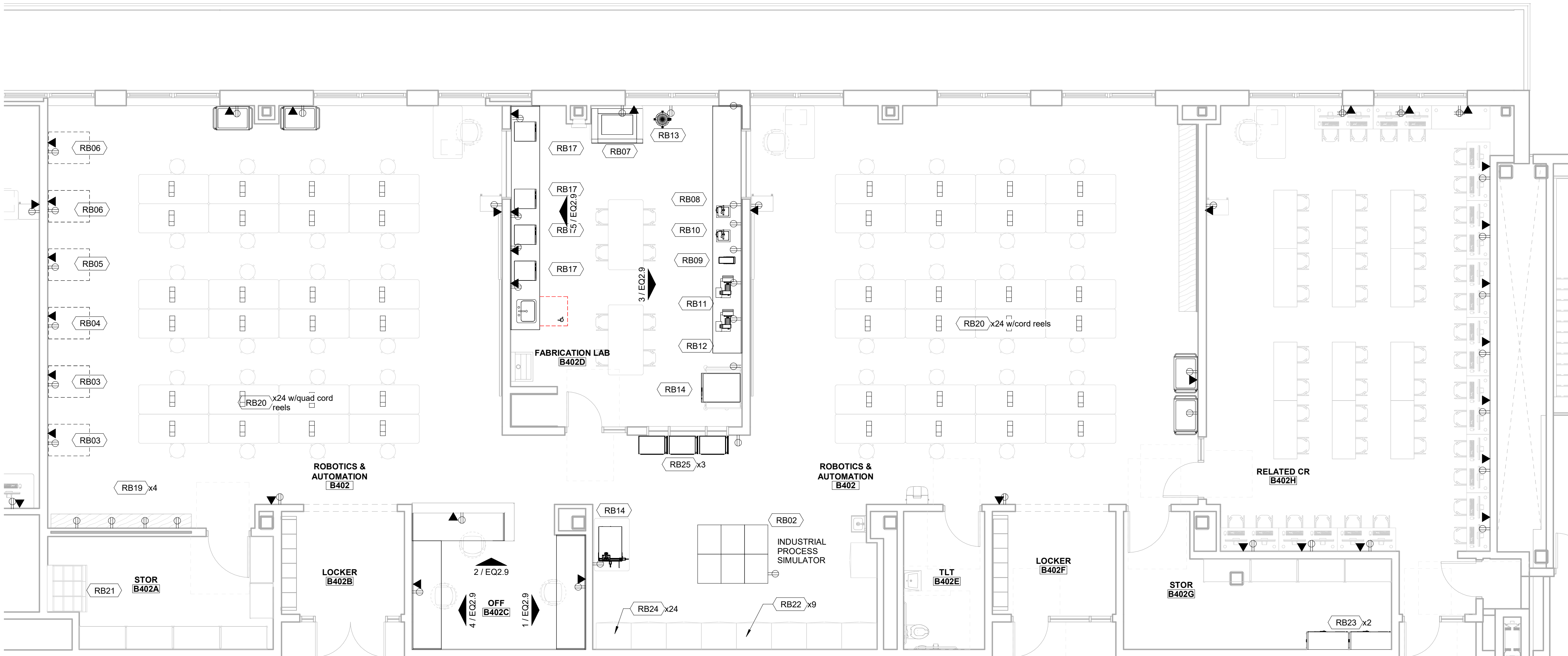
6 Level 4 - Robotics 3/16" = 1'-0"
