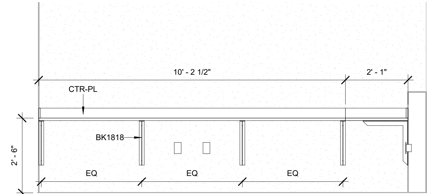
6 A402G - Dental Assist, Office, West 1/2" = 1'-0"
