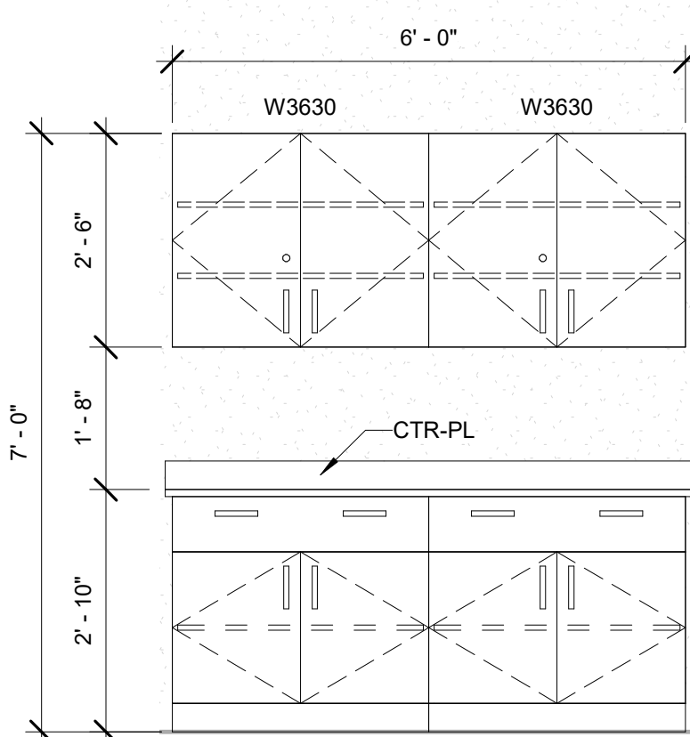
22 A404E - SUP ASSIST 1/2" = 1'-0"
