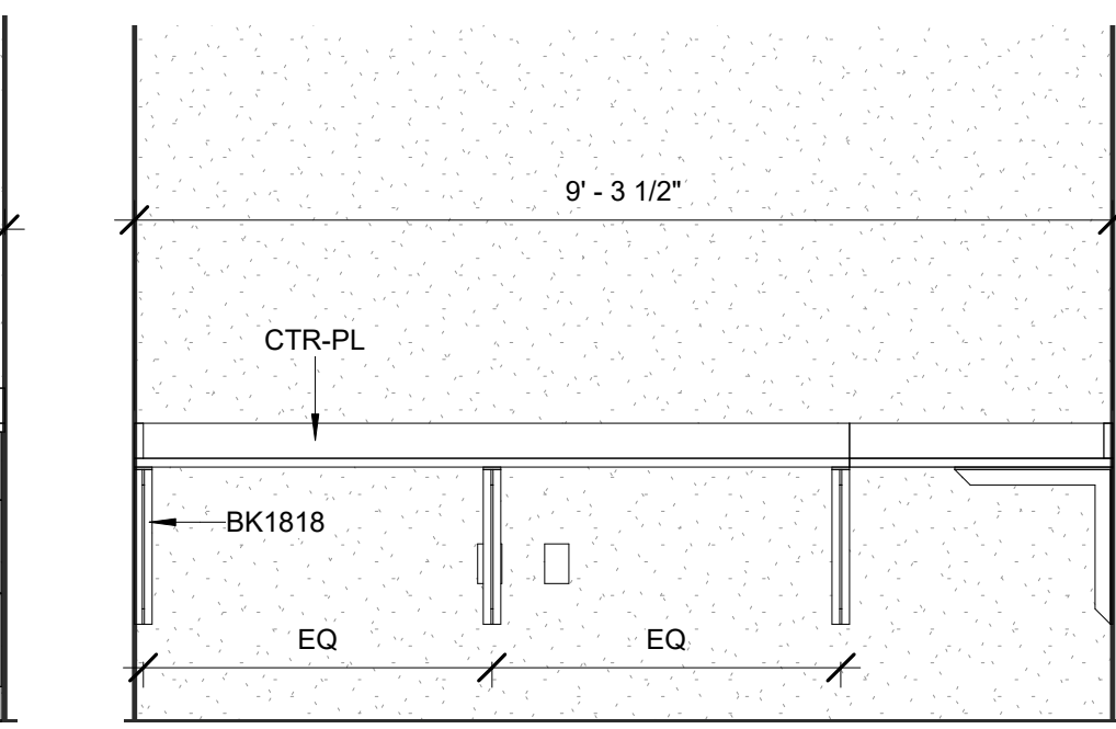
6 A303D - BioTech - Office - East 1/2" = 1'-0"
