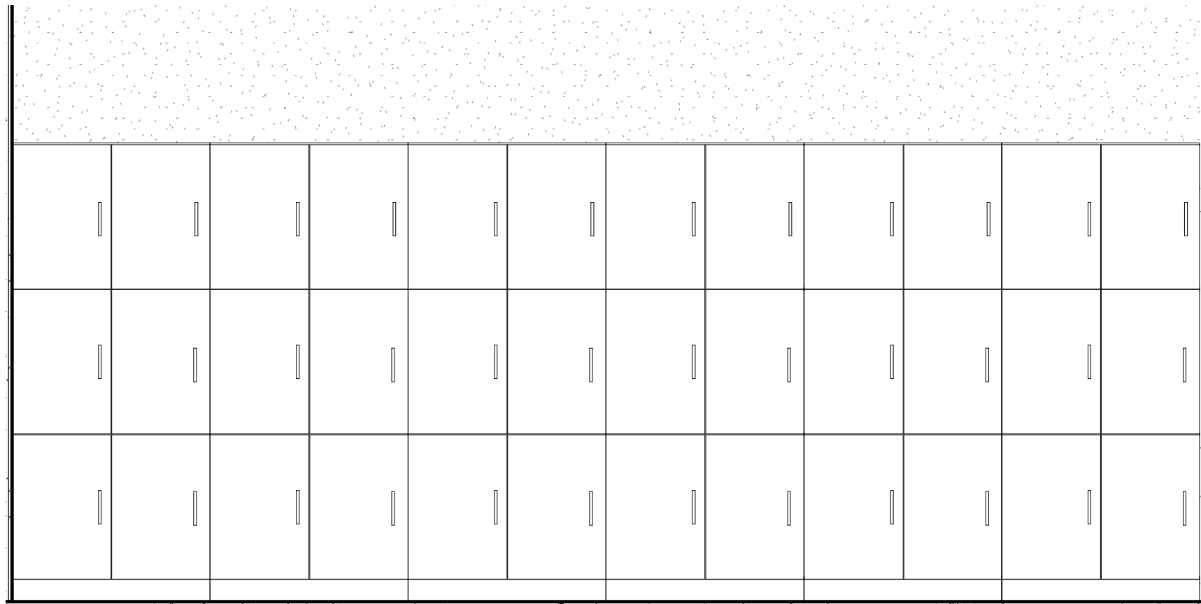
1 B120 - Cosmetology Lockers 1/2" = 1'-0"
