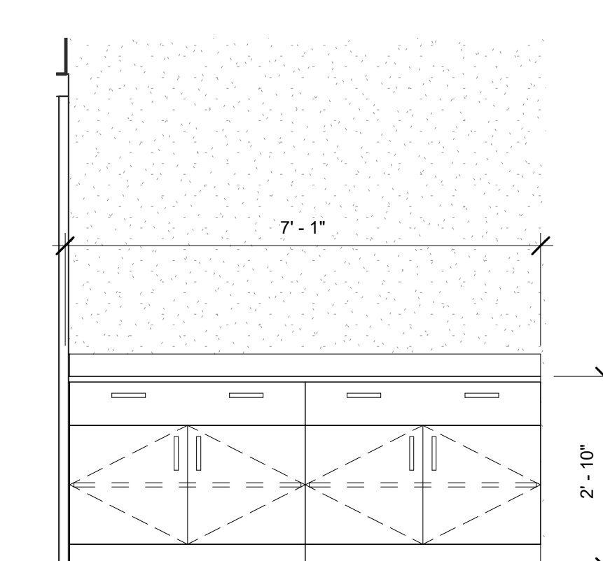
12 A303H - BioTech - Lab - West 1/2" = 1'-0"
