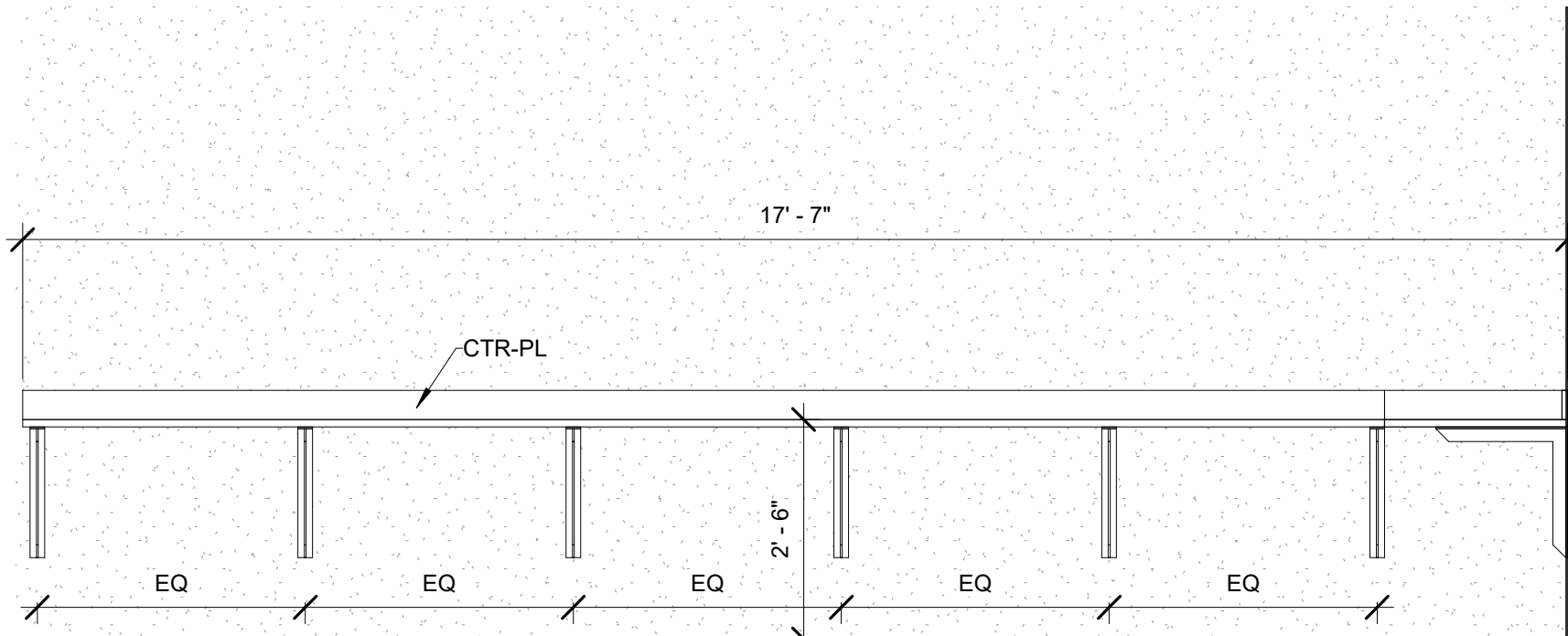
3 B201E- Drafting and Design- Office- East 1/2" = 1'-0"
