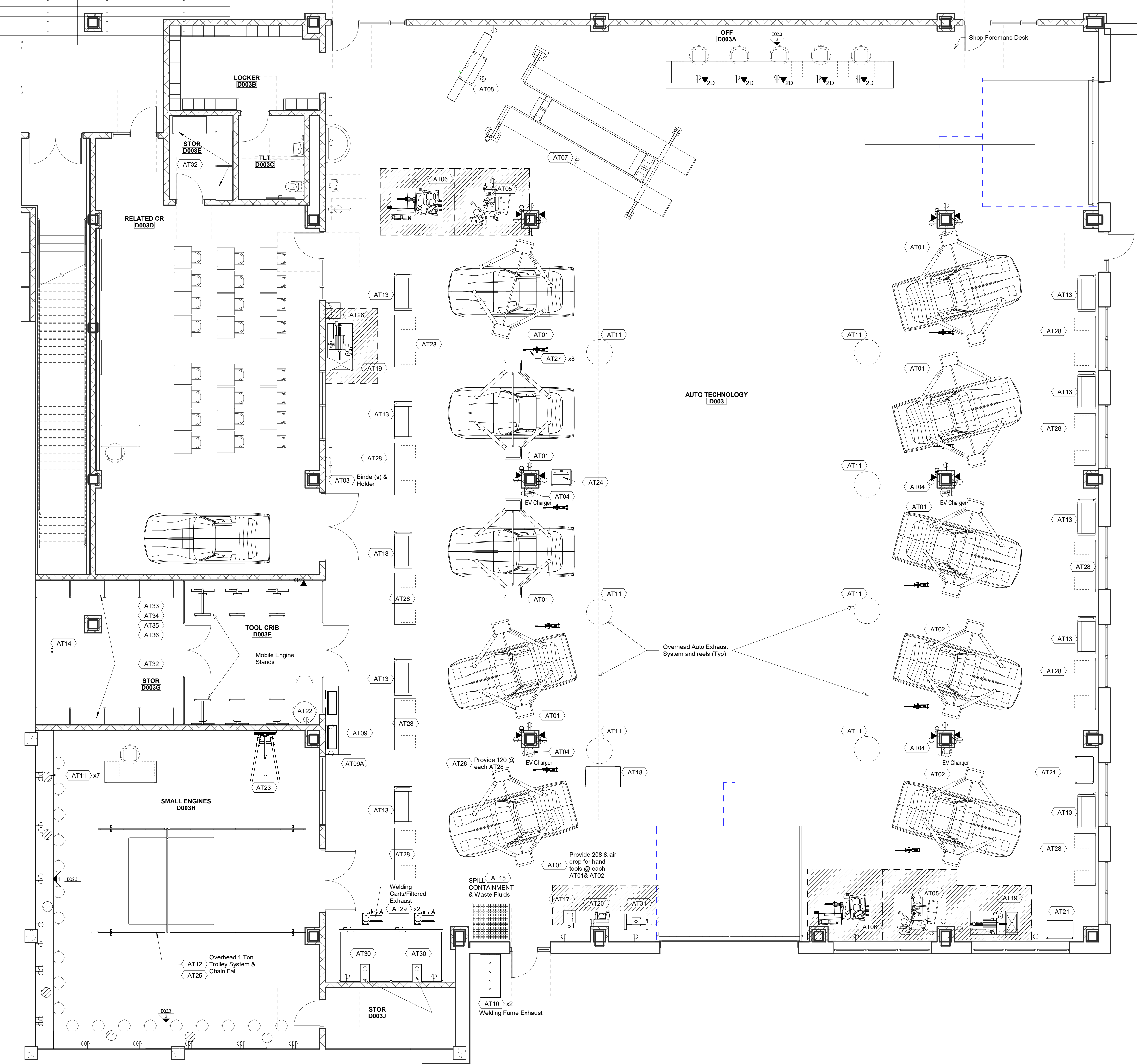
4 Level 0 - Auto Tech 3/16" = 1'-0"
