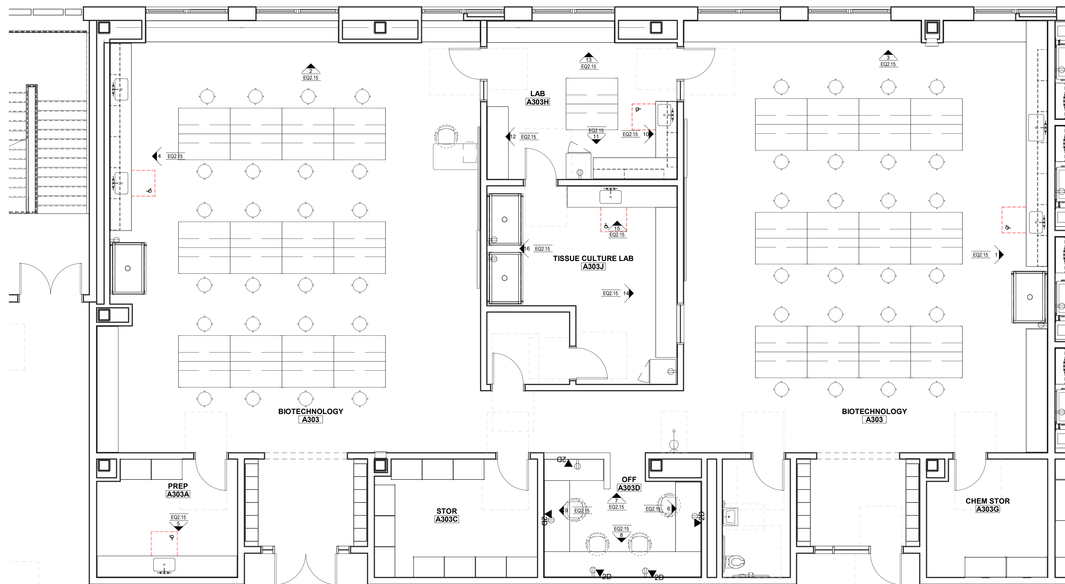
25 Level 3 - BioTech 3/16" = 1'-0"
