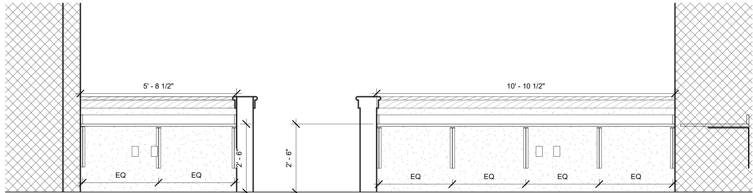
1 A141F - Carpentry - Staff Office - North 1/2" = 1'-0"
