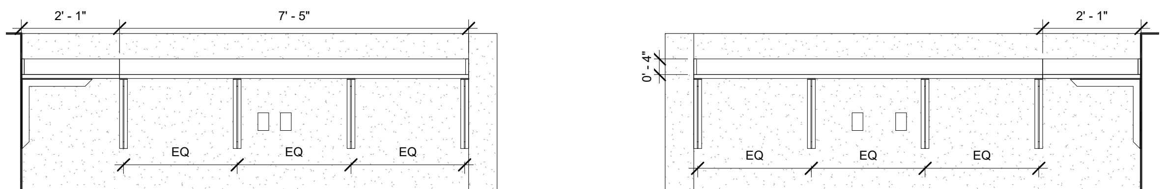
3 B103-Hvac- Office- East 1/2" = 1'-0"
