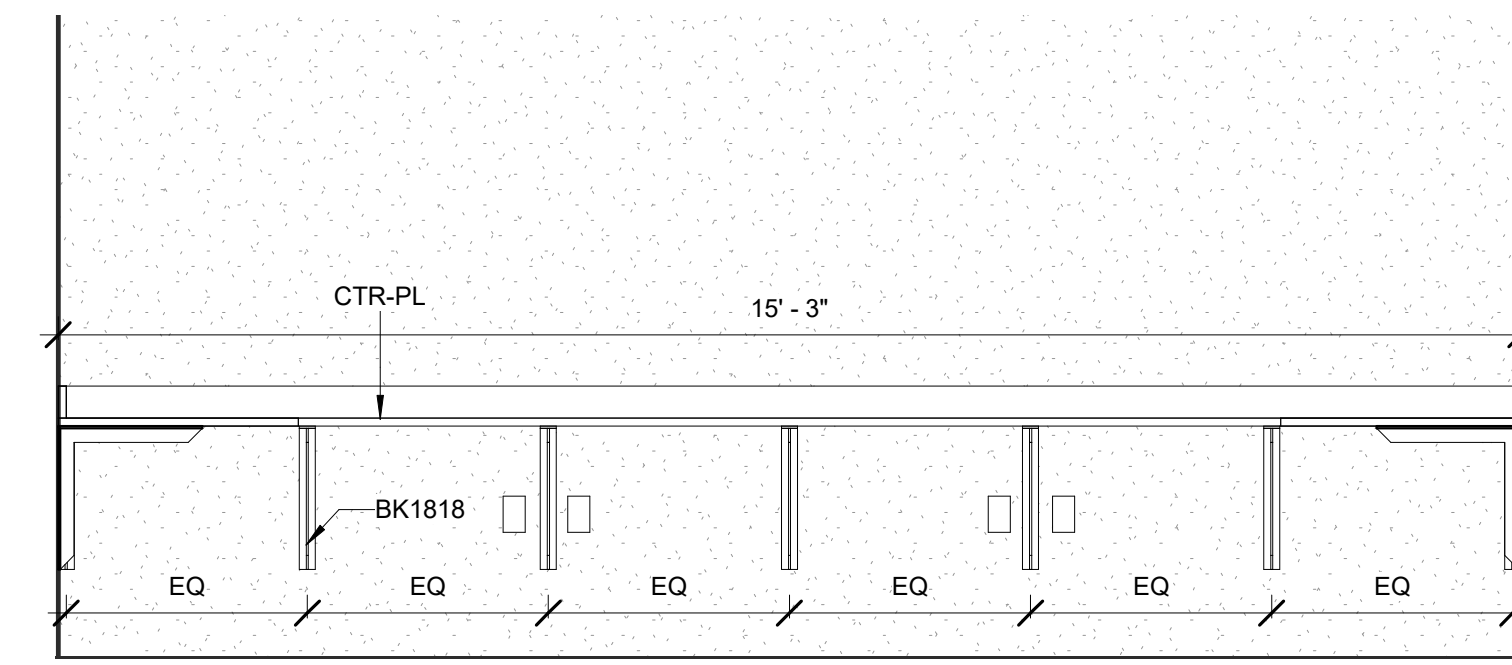
8 A303D - BioTech - Office - South 1/2" = 1'-0"
