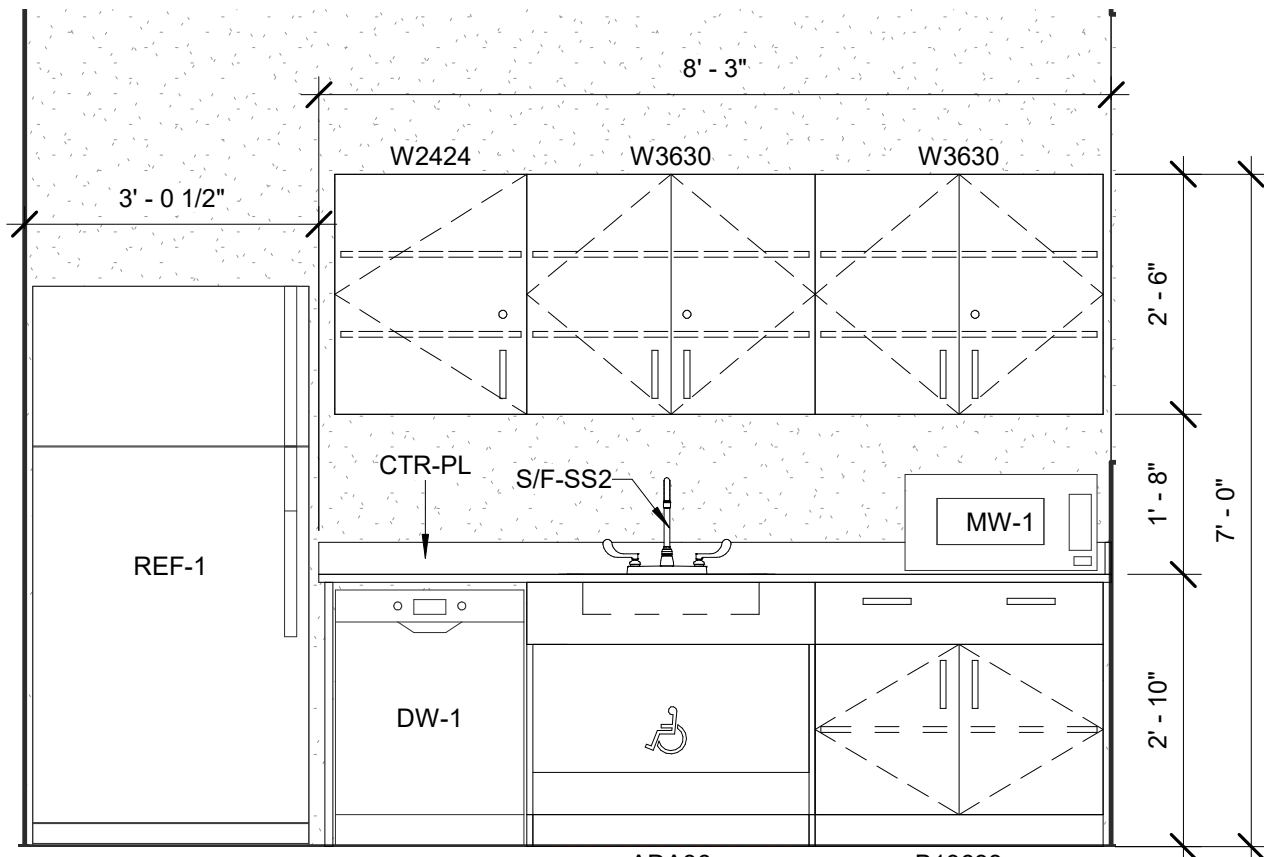
18 C106J - Kitchen, North 1/2" = 1'-0"
