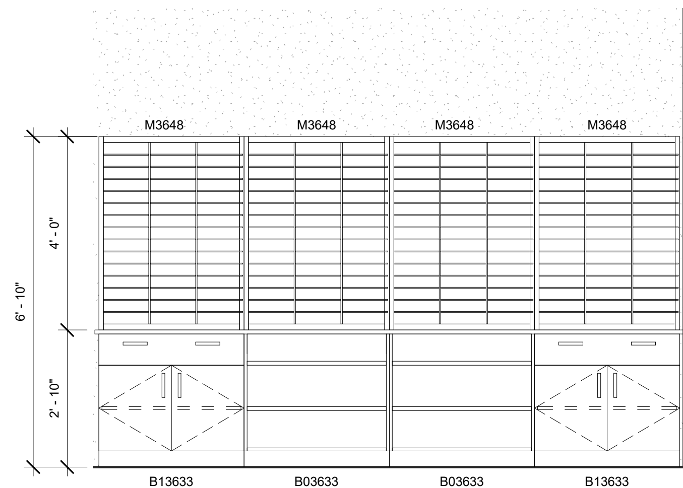
15 A139 - Mail, North 1/2" = 1'-0"
