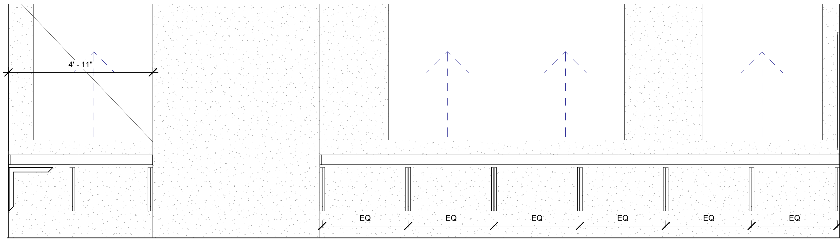
8 B202C - Computer Lab, North 1/2" = 1'-0"
