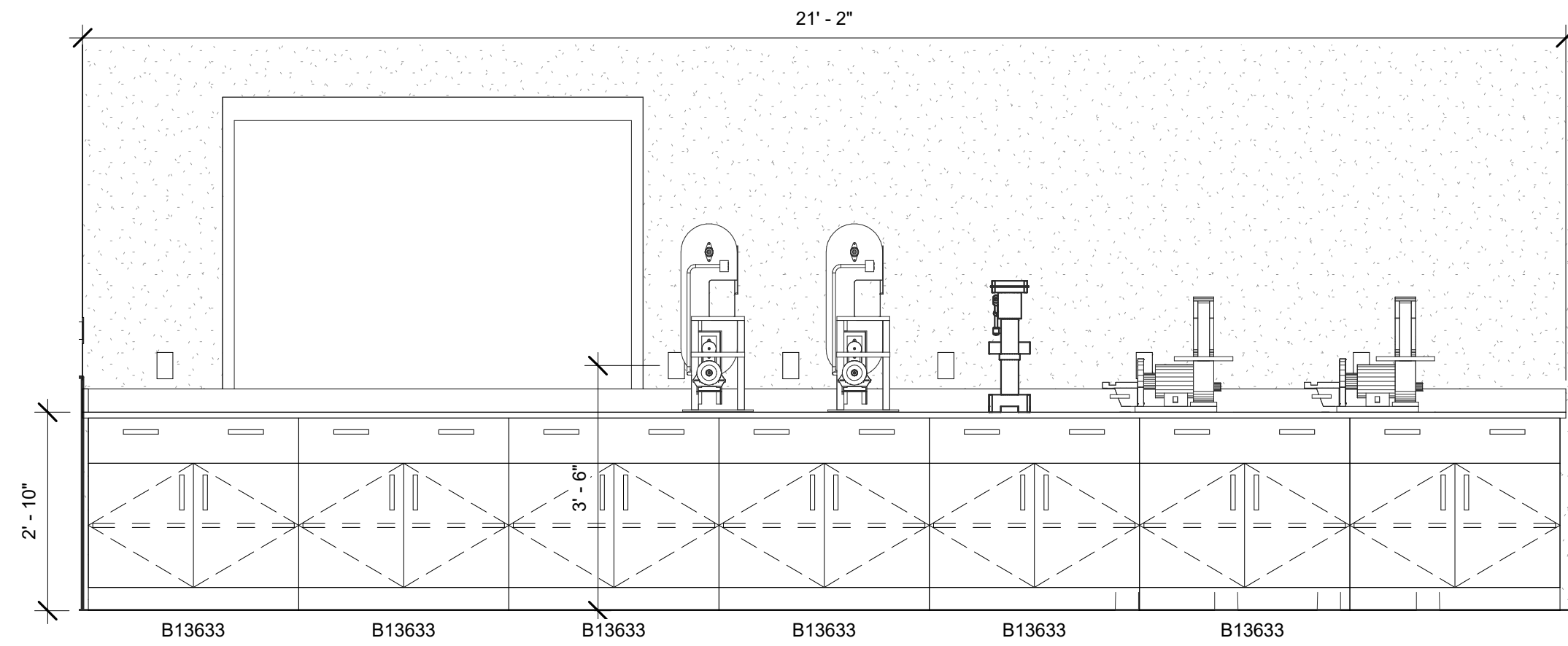
3 B368- Fabrication Lab- East 1/2" = 1'-0"
