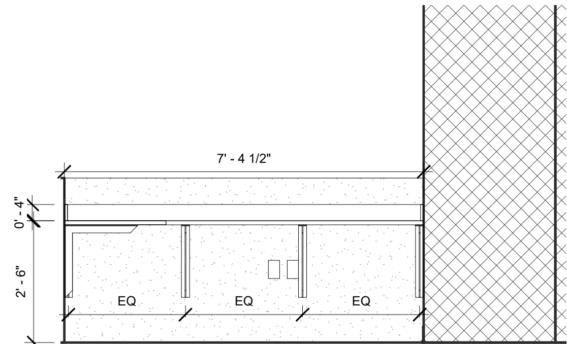
2 B101F - Plumbing - Staff Office, North 1/2" = 1'-0"
