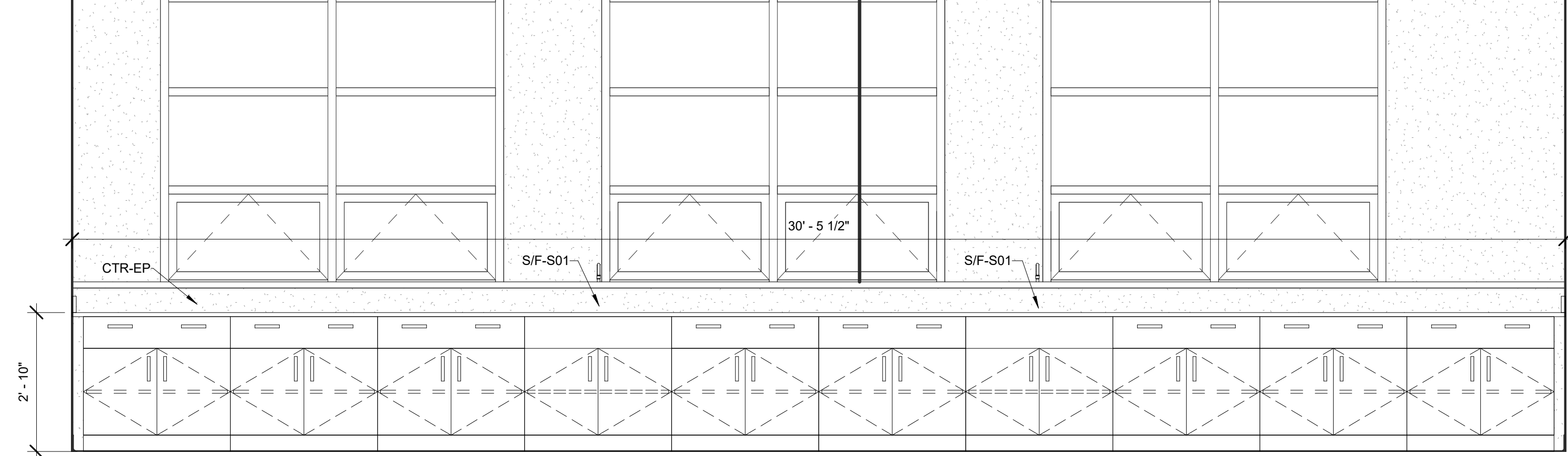
3 Science Lab - Typical @ Window Wall 1/2" = 1'-0"
