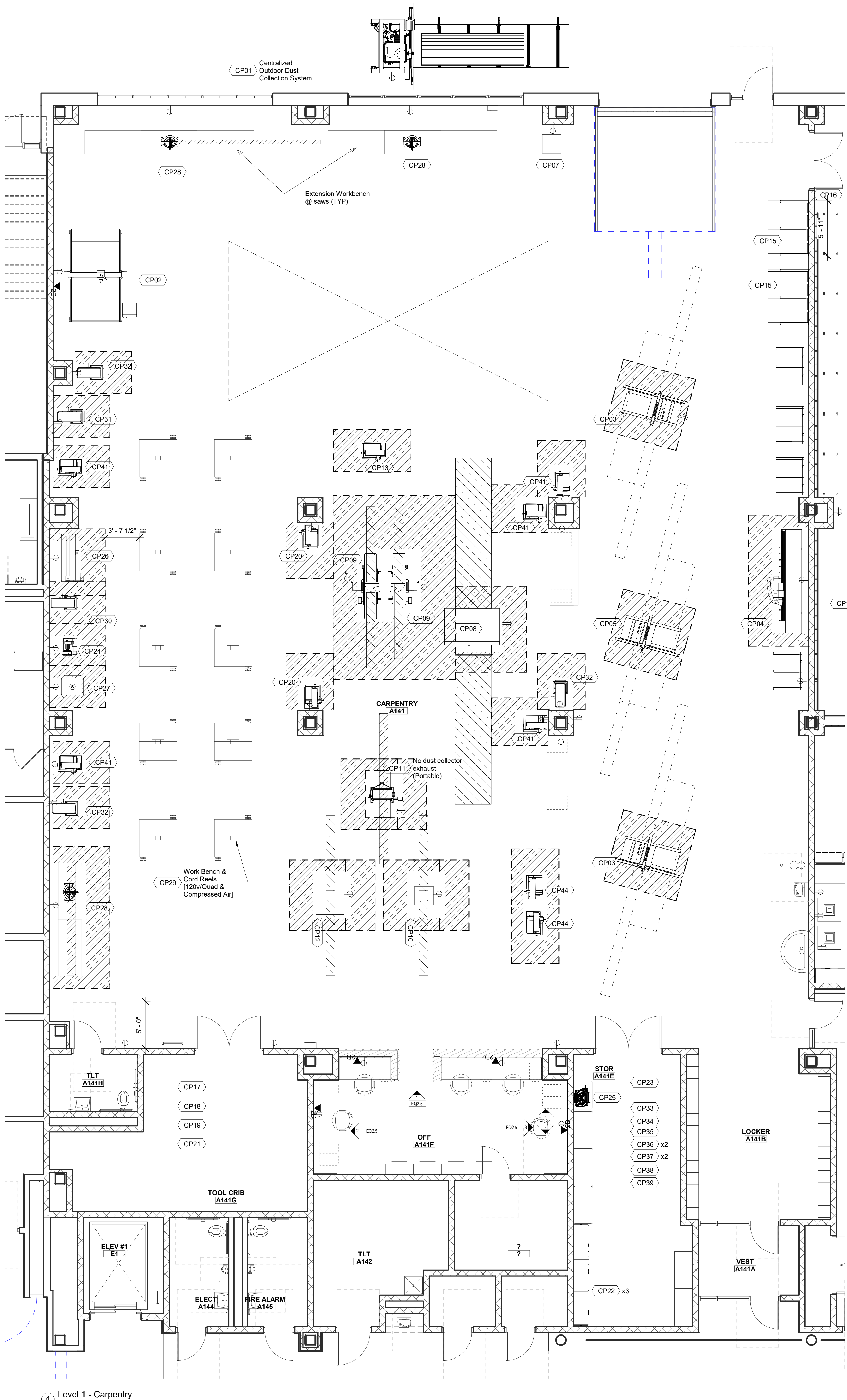
4 Level 1 - Carpentry 3/16" = 1'-0"
