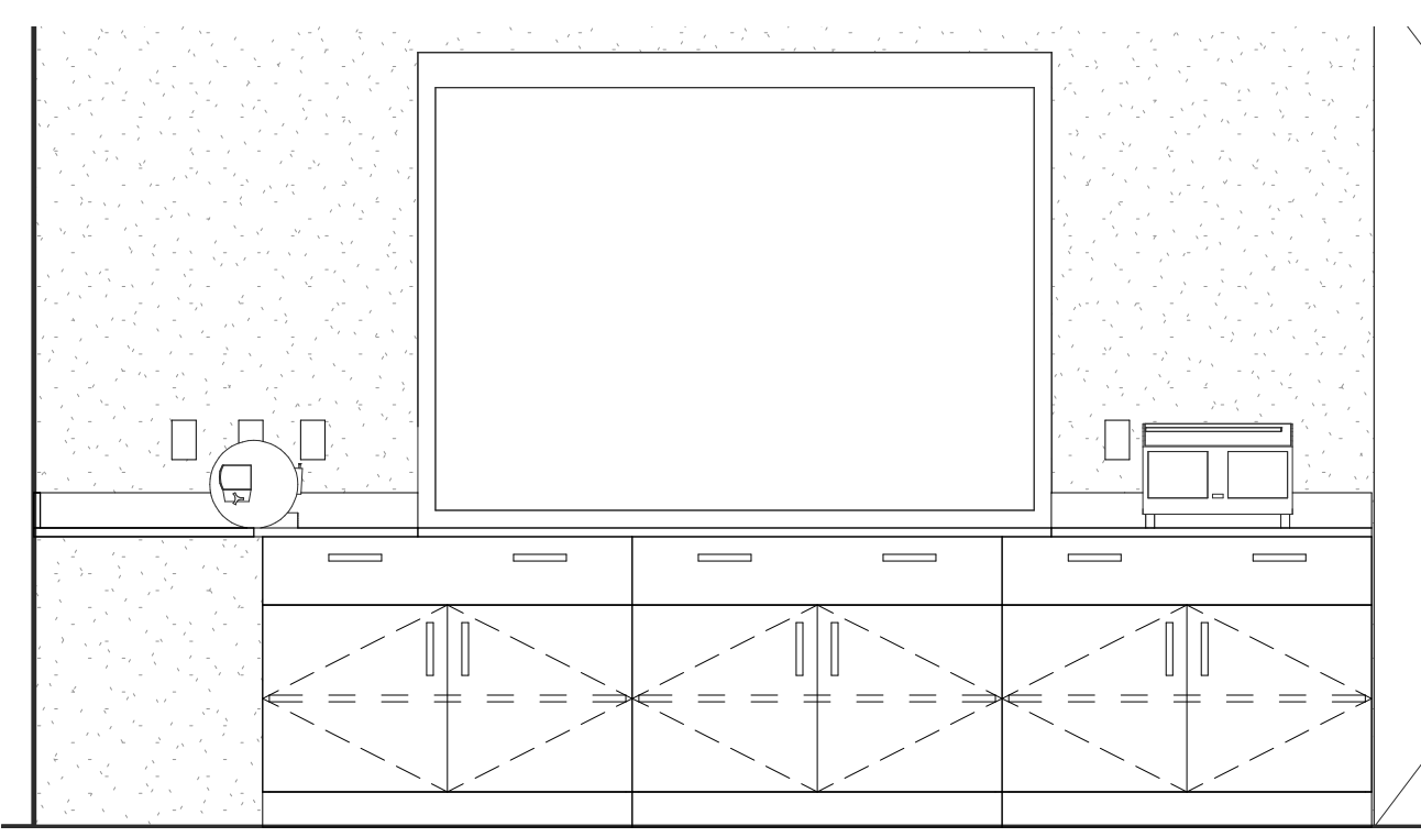
② A402B - Model Making, North 1/2" = 1'-0"
