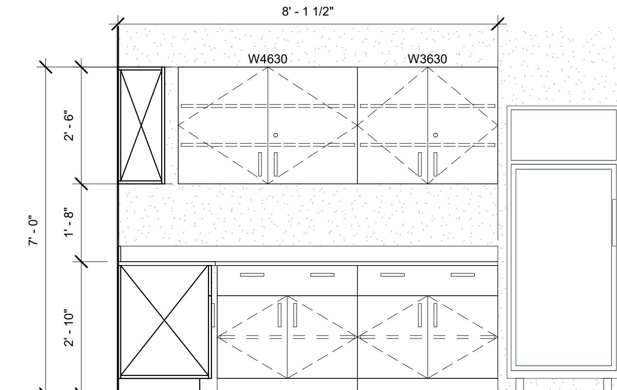
11 A303H - BioTech - Lab - South 1/2" = 1'-0"
