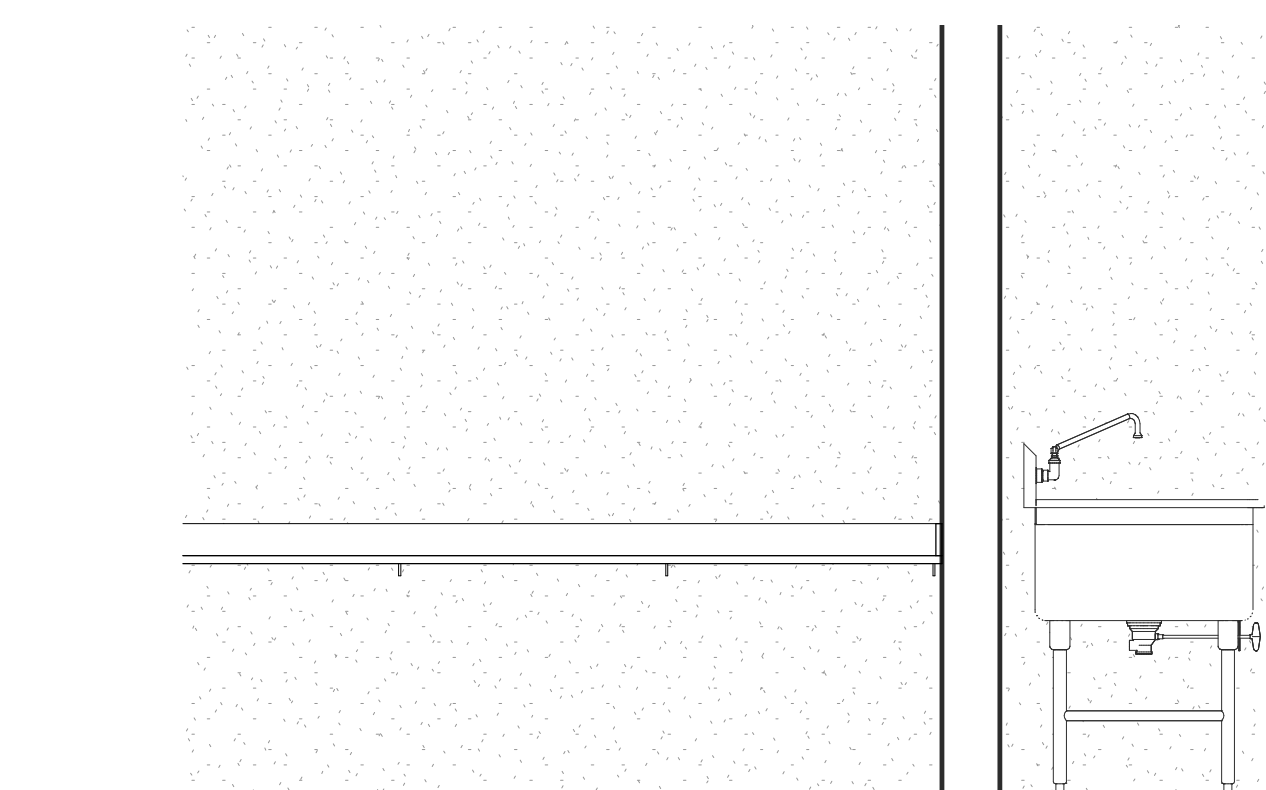
17 A148G - Culinary Office, East 1/2" = 1'-0"
