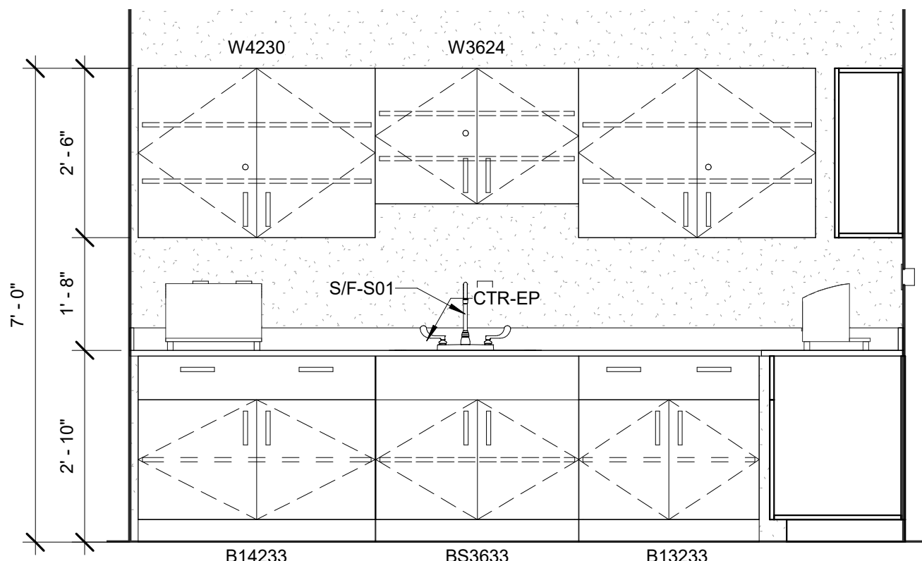
⑥ A402P - Model Making, East 1/2" = 1'-0"
