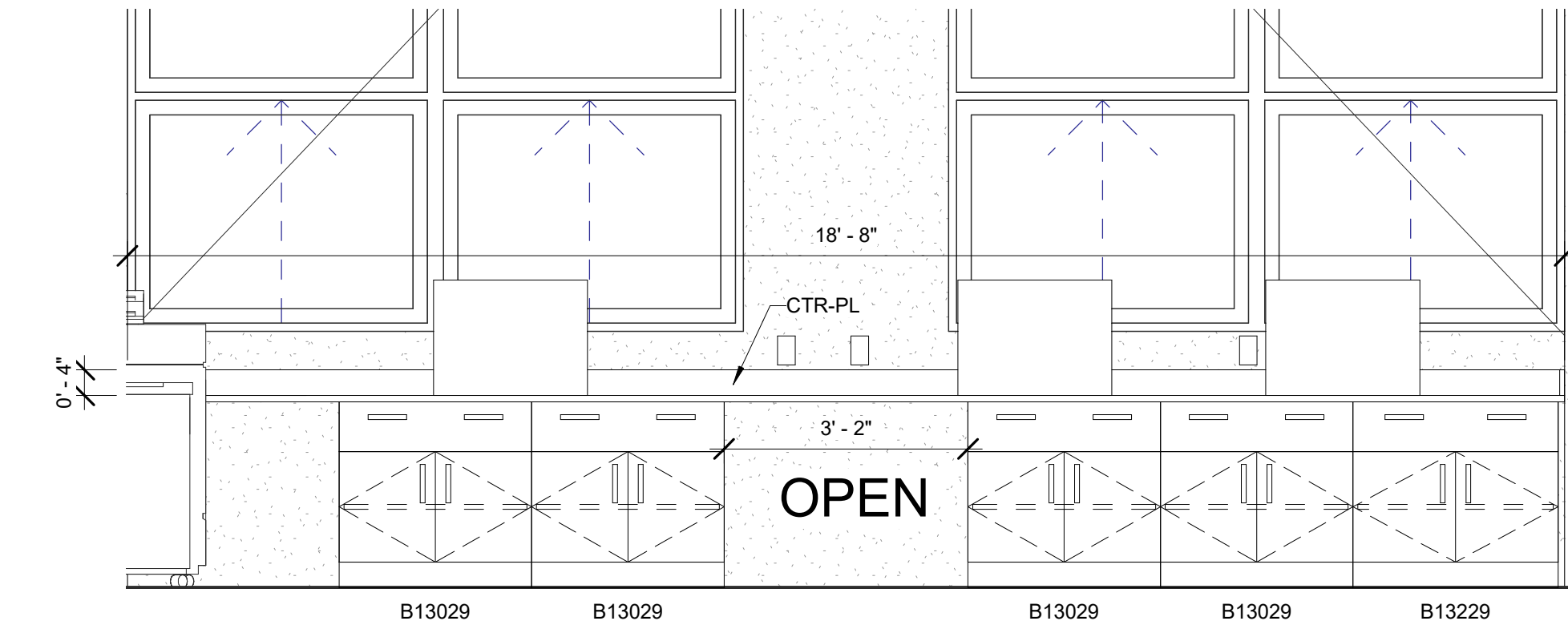
2 A206 - Design- Visual Comm, North 1/2" = 1'-0"
