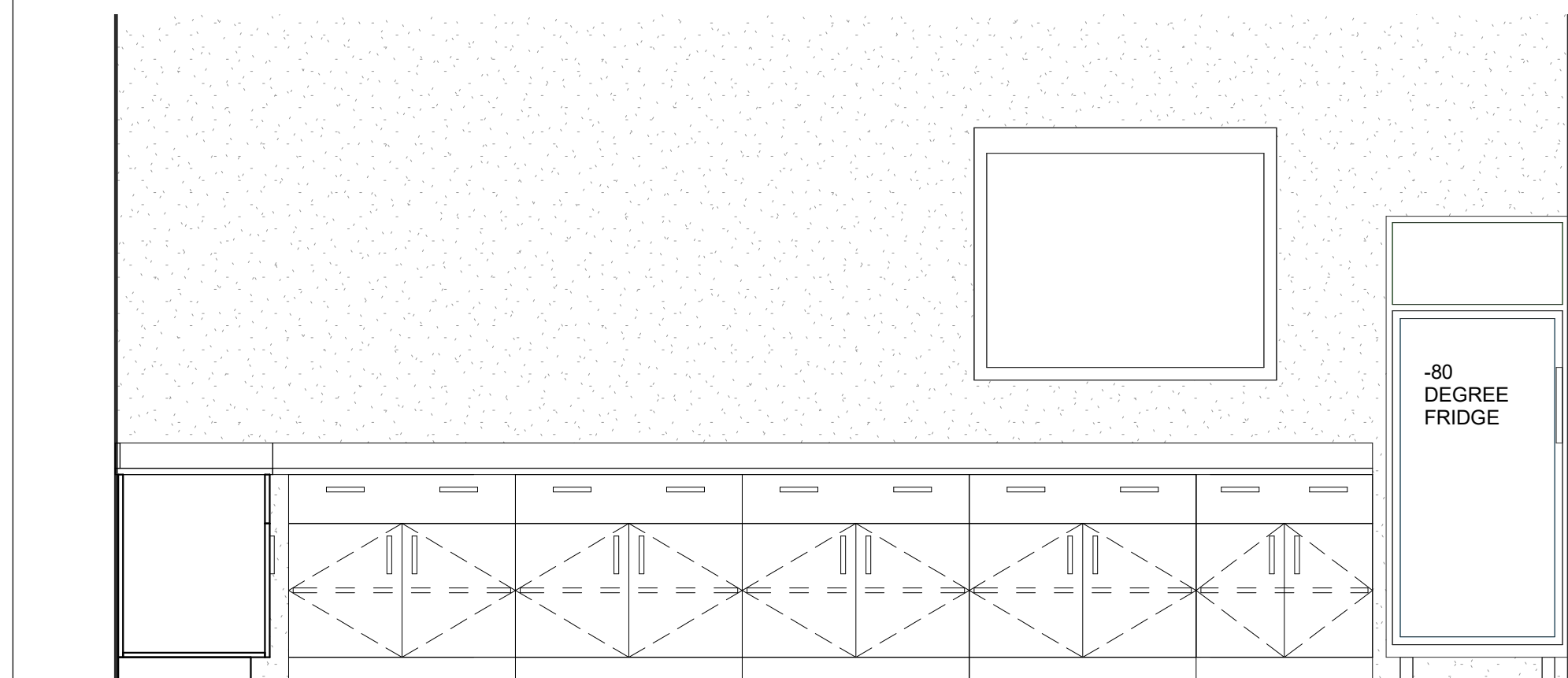
14 A303J - BioTech - Tissue Culture Lab - East 1/2" = 1'-0"
