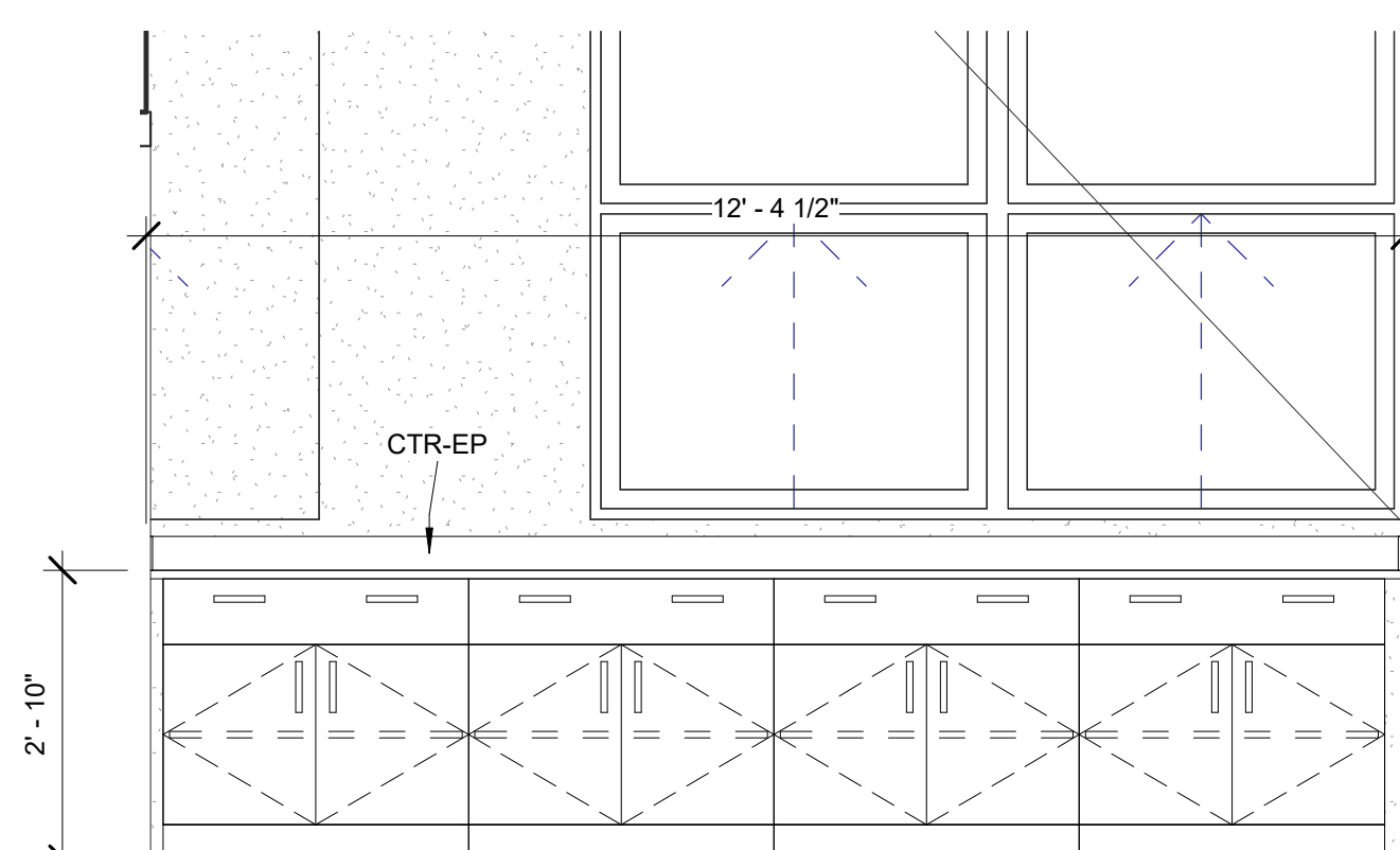
13 A303H - BioTech - Lab - North 1/2" = 1'-0"
