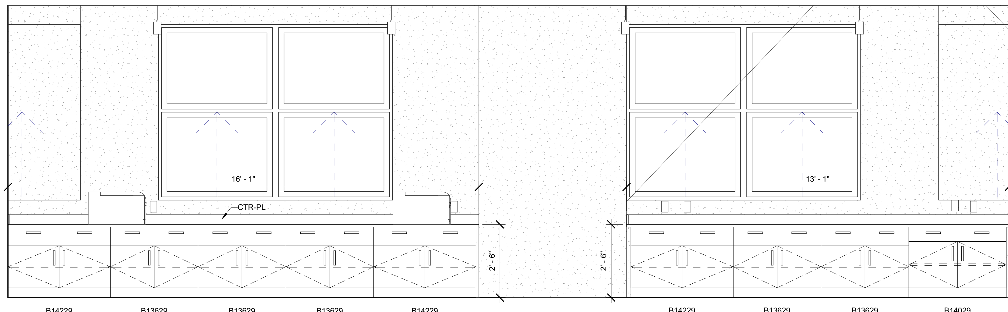
7 B201D - Computer Lab, North 1/2" = 1'-0"
