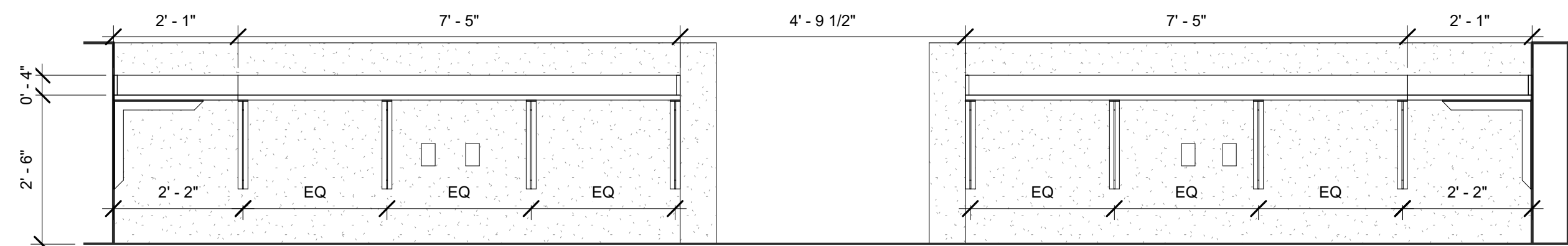
3 B101F - Plumbing - Staff Office, West 1/2" = 1'-0"
