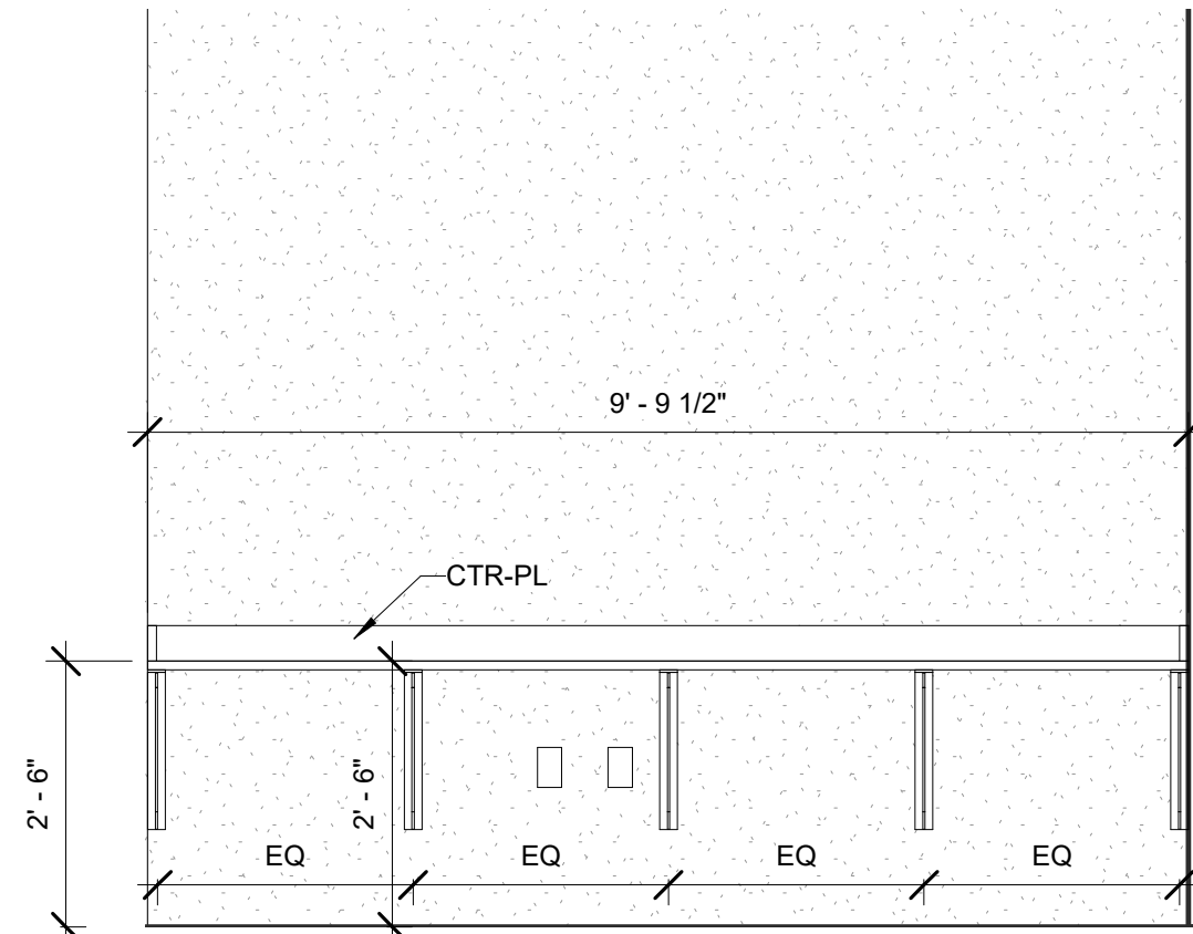
1 B369- Robotics- Office- East 1/2" = 1'-0"
