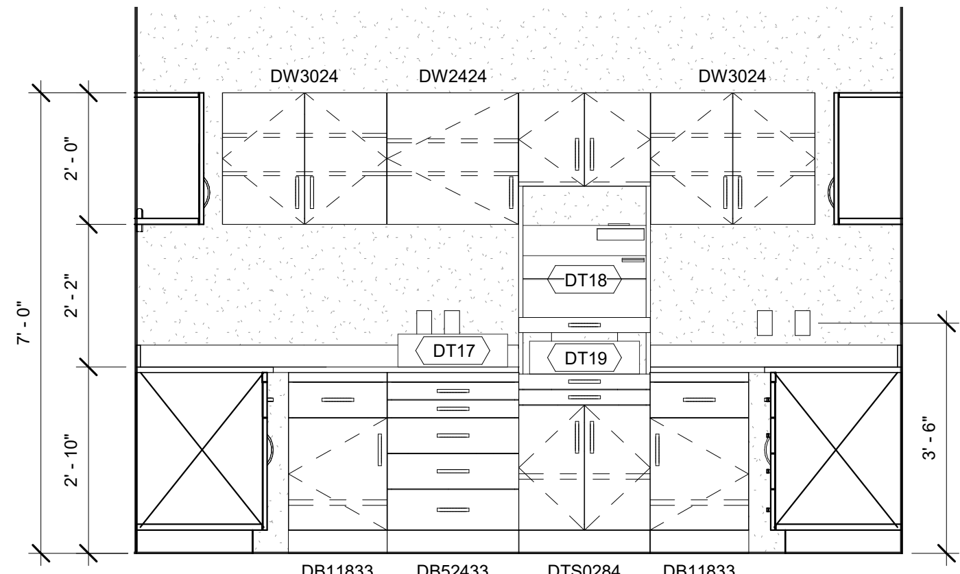
⑨ A402D - Steralization, South 1/2" = 1'-0"
