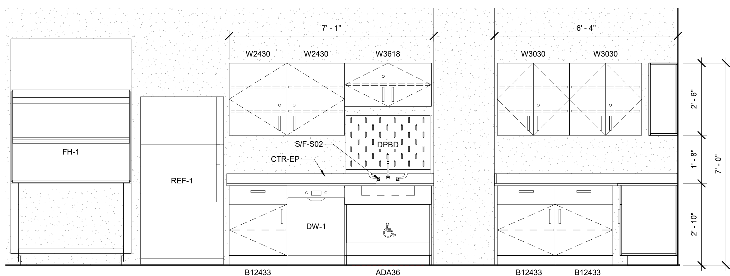
9 B316 - SCI PREP, South 1/2" = 1'-0"
