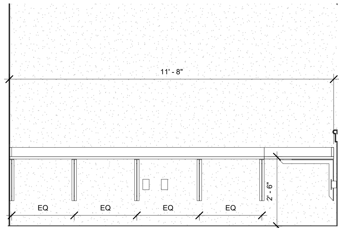
4 B369- Robotics- Office- West 1/2" = 1'-0"
