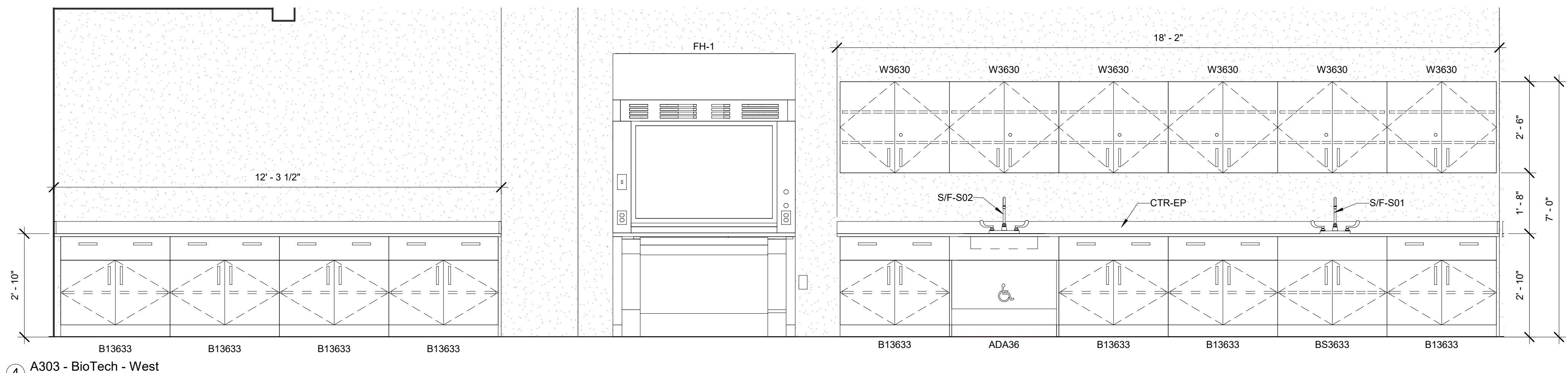
4 A303 - BioTech - West 1/2" = 1'-0"
