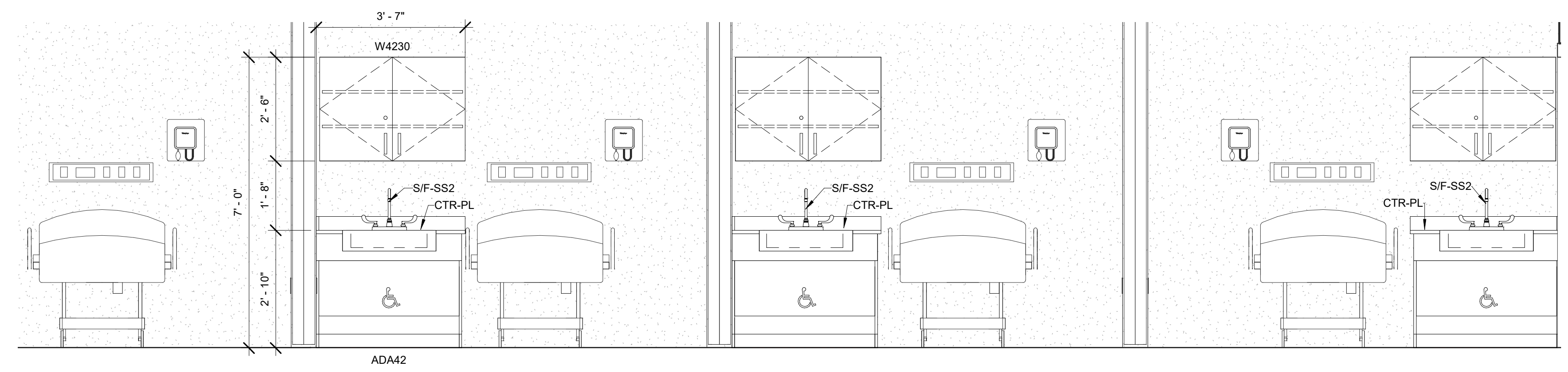
② B301 - Health Assist - East 1/2" = 1'-0"
