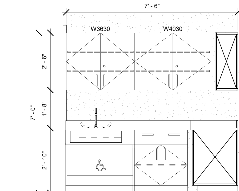
10 A303H - BioTech - Lab - East 1/2" = 1'-0"
