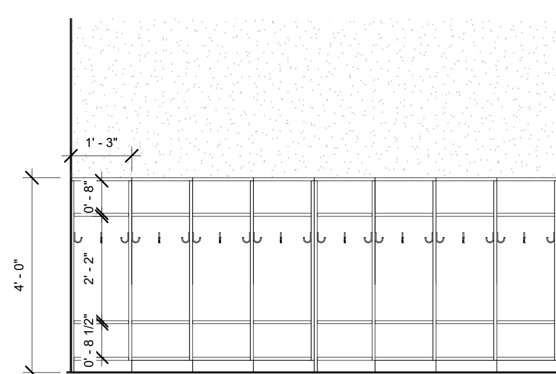
16 C106A - CUBBIES, North 1/2" = 1'-0"
