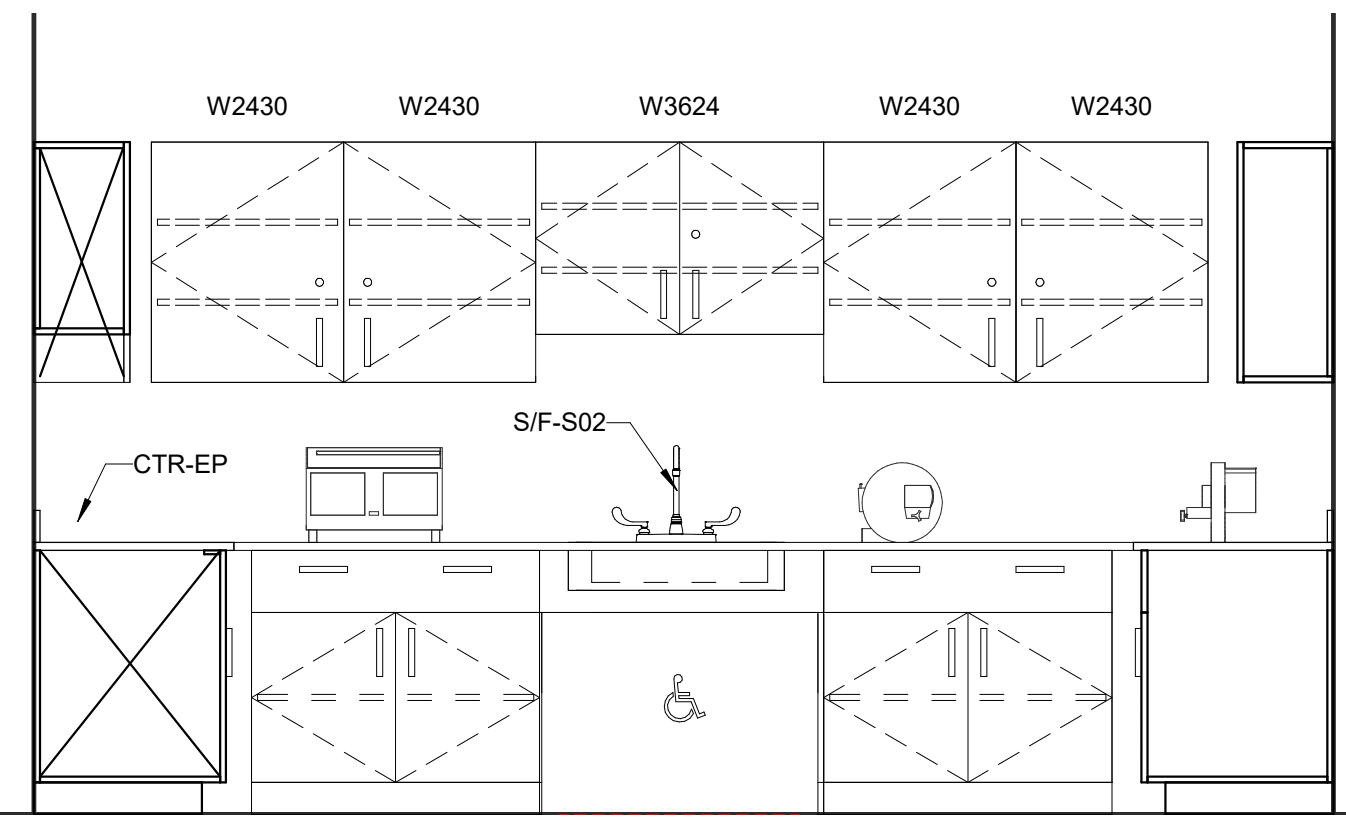
⑤ A402P - Model Making, South 1/2" = 1'-0"
