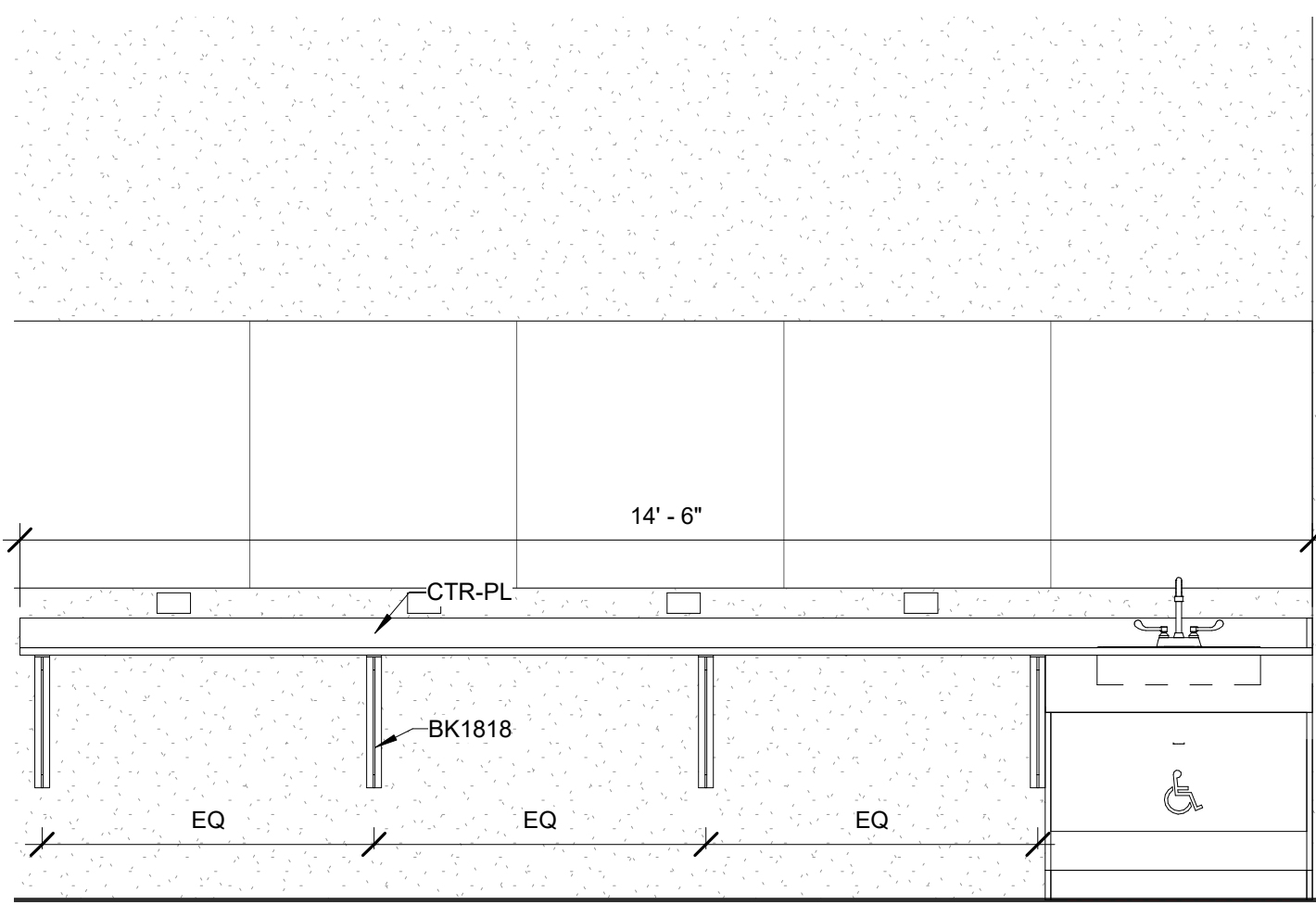
21 C110 - Dressing, North 1/2" = 1'-0"
