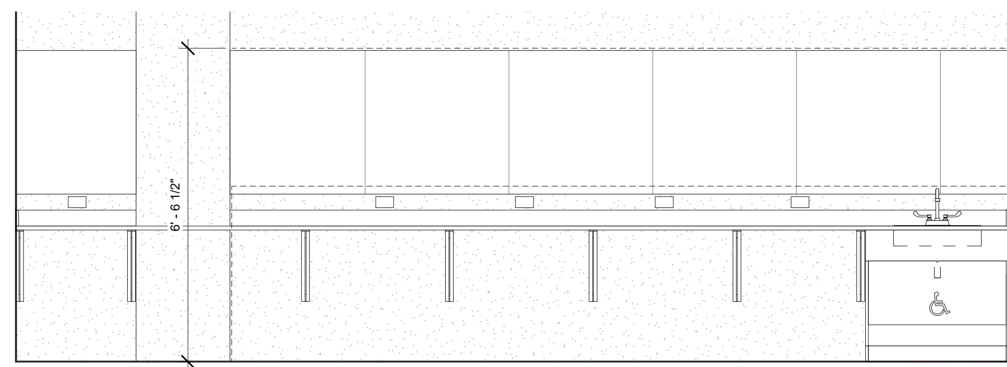
20 C107 - Dressing, North 1/2" = 1'-0"
