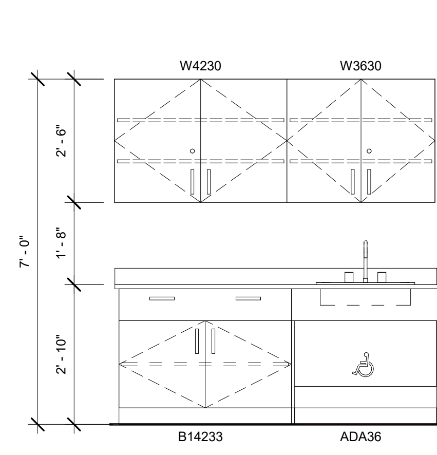
3 D110 - Nurse - Exam 1/2" = 1'-0"
