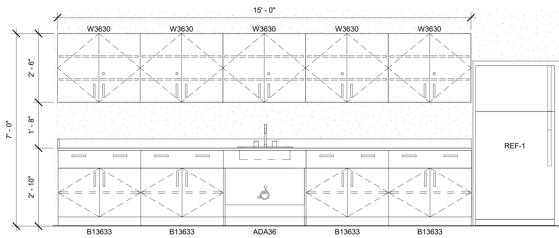
14 A131 - Duplicating - East 1/2" = 1'-0"
