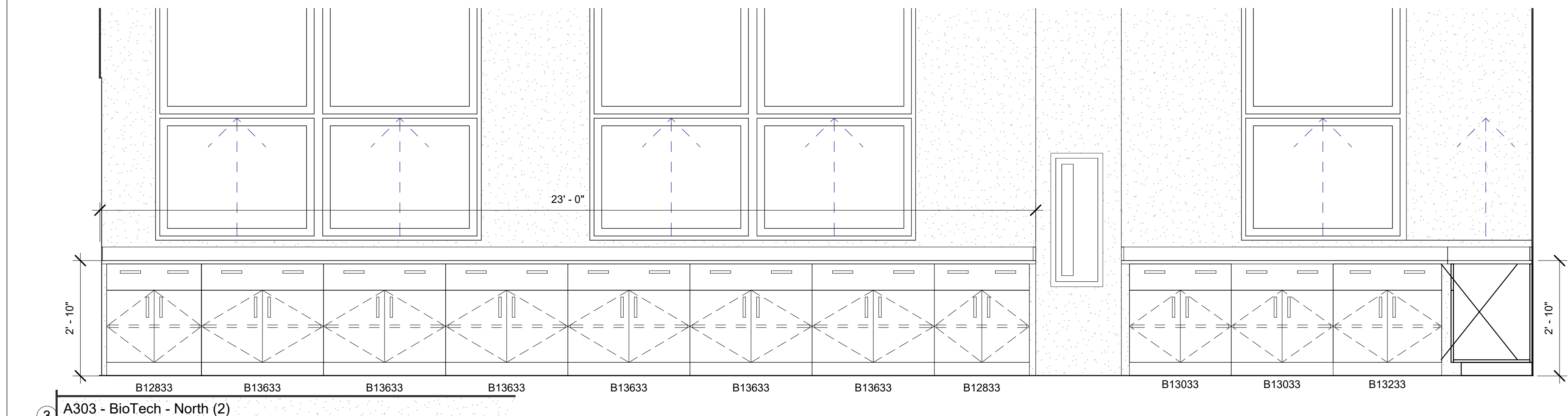
3 A303 - BioTech - North (2) 1/2" = 1'-0"
