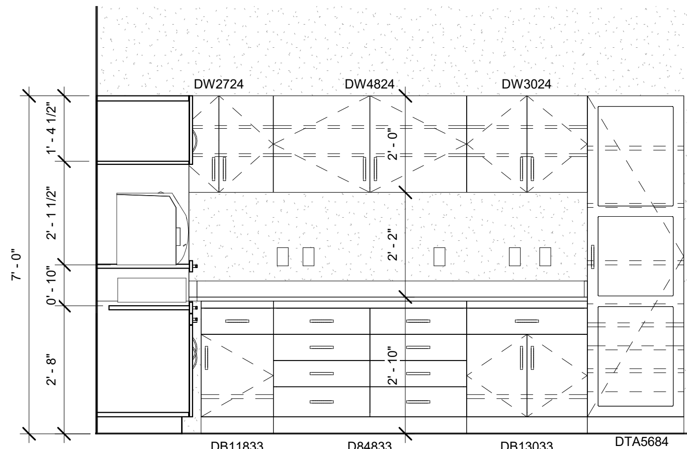
⑩ A402D - Steralization, West 1/2" = 1'-0"
