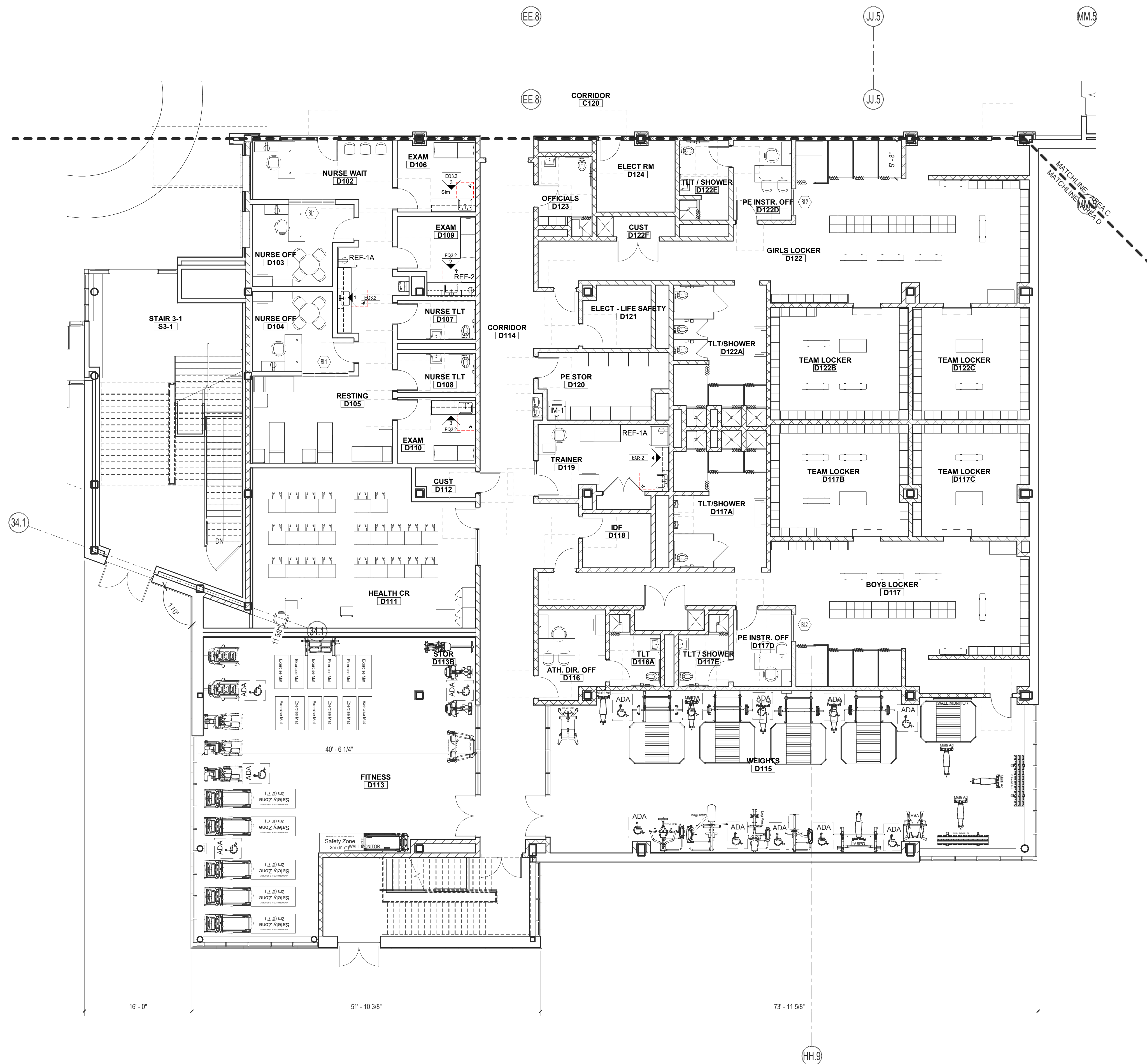
1 Level 1 - Area D 1/8" = 1'-0"
