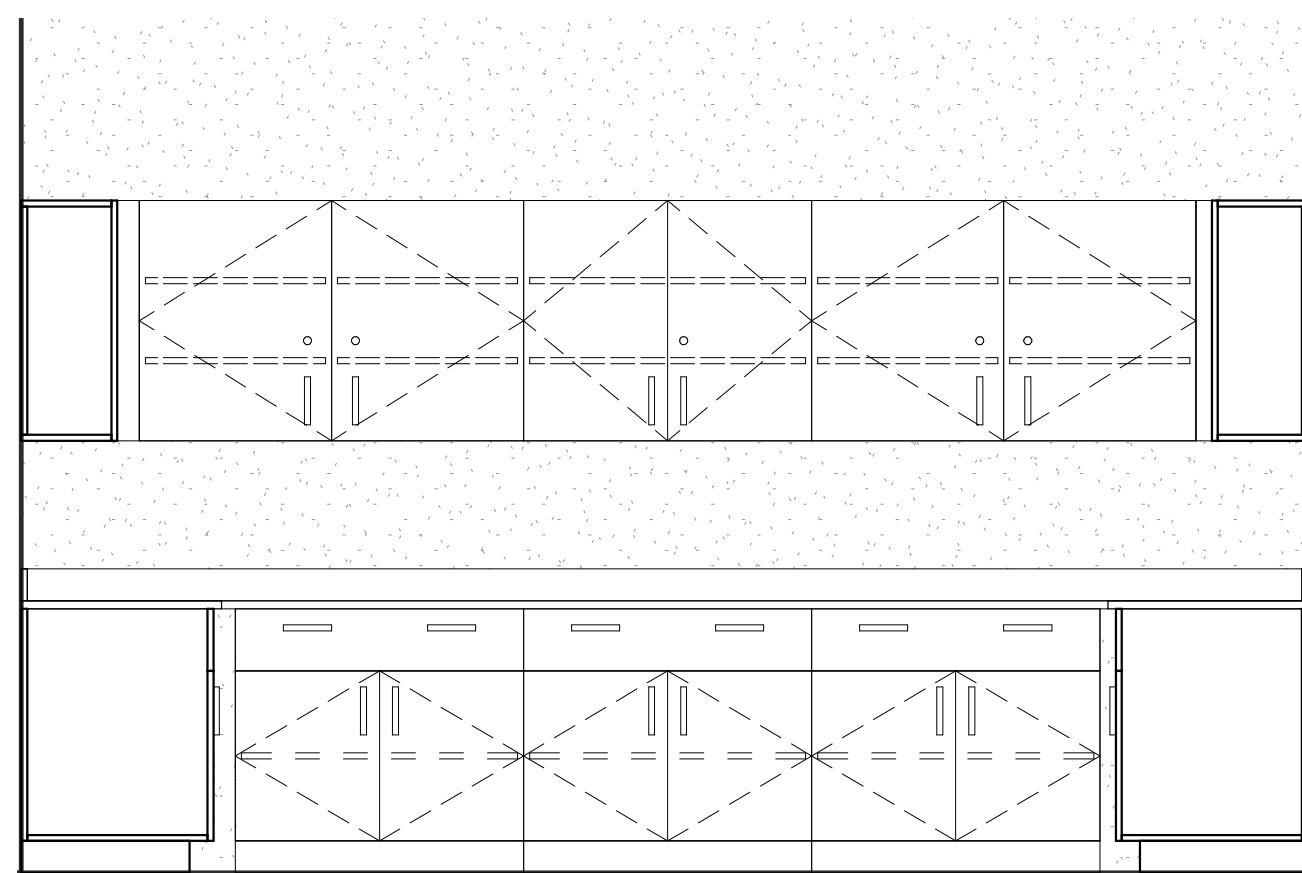
6 Science Prep - Typical for East or West 1/2" = 1'-0"
