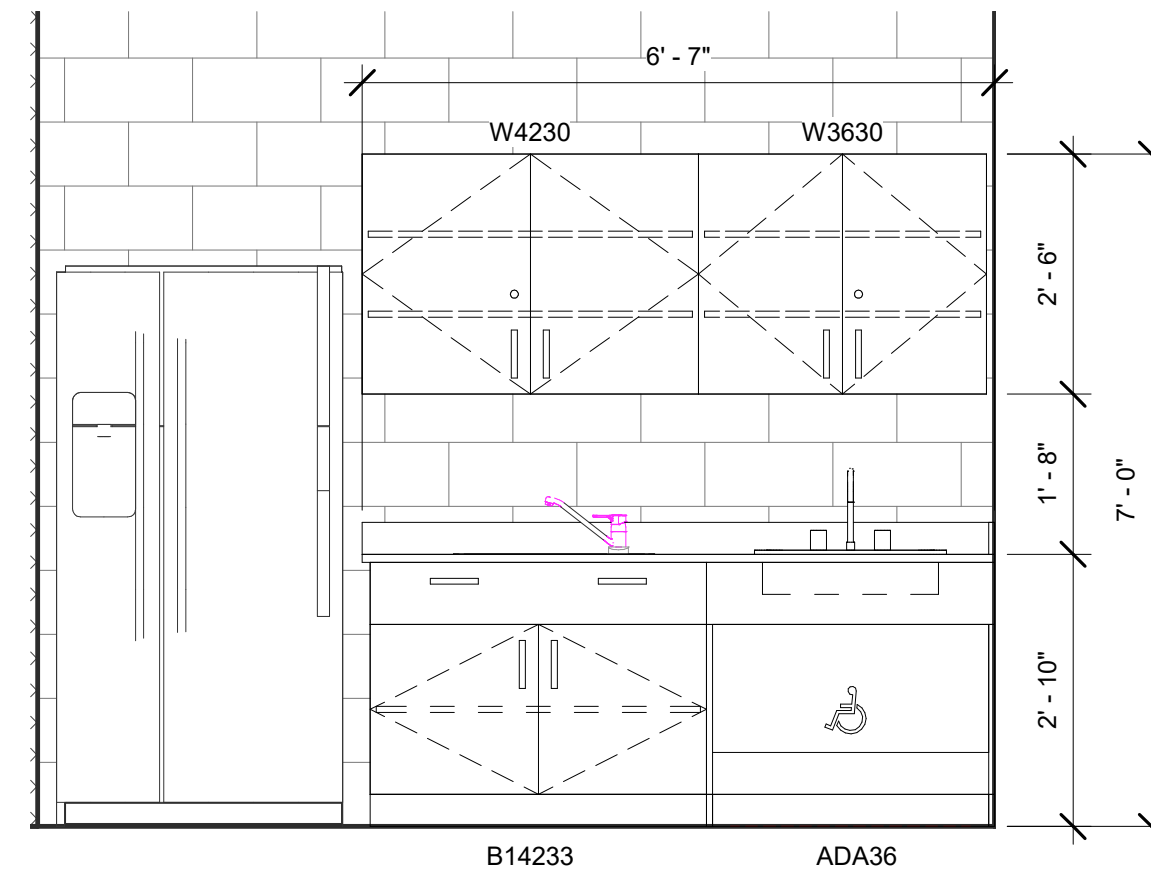
4 D119 - Trainer, East 1/2" = 1'-0"
