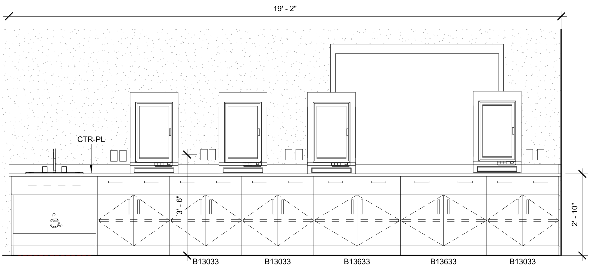
5 B368- Fabrication Lab- West 1/2" = 1'-0"
