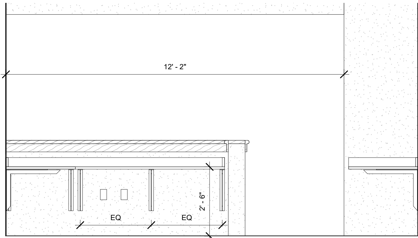
2 B369- Robotics- Office- North 1/2" = 1'-0"
