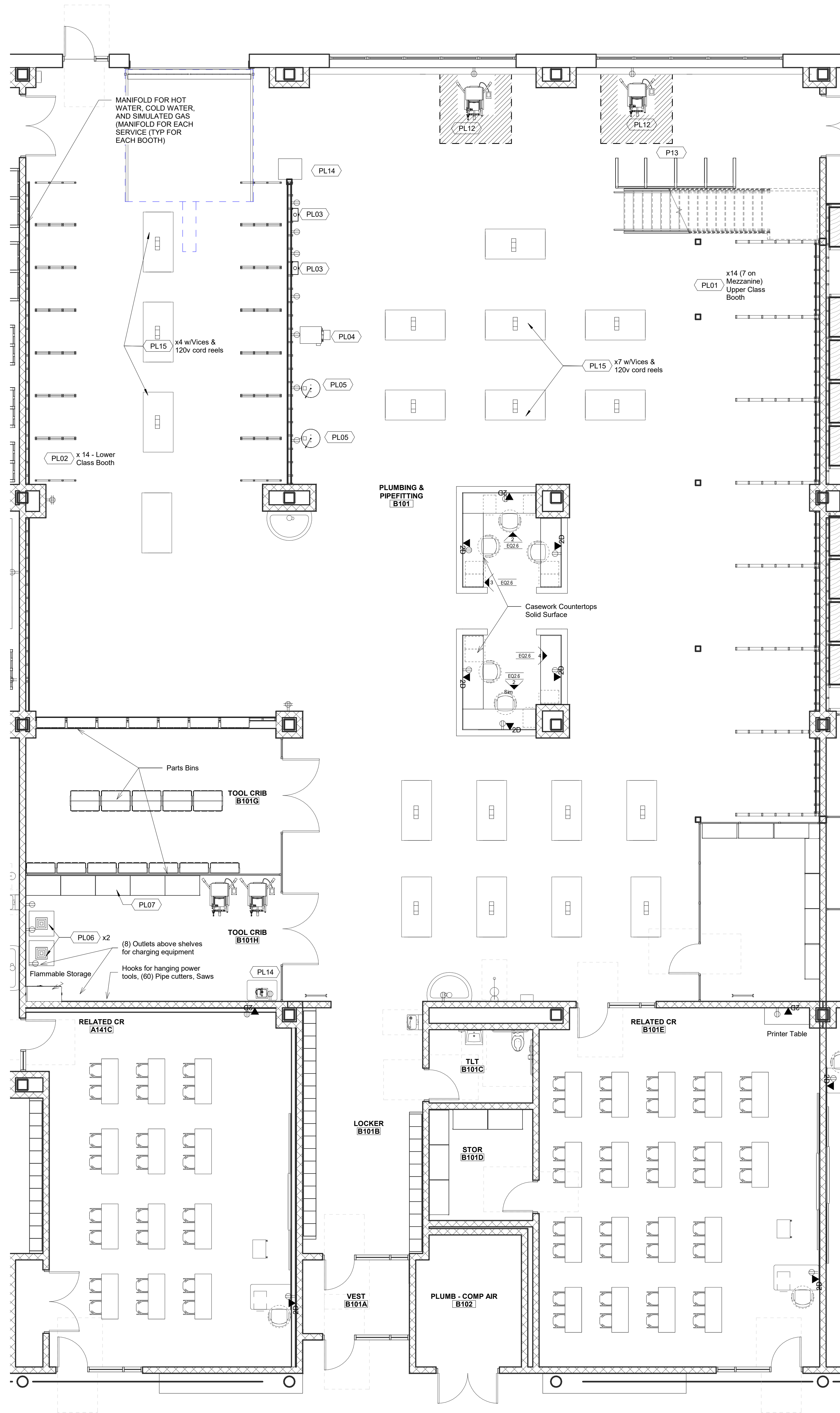
1 Level 1 - Plumbing - Pipe Fitting 3/16" = 1'-0"
