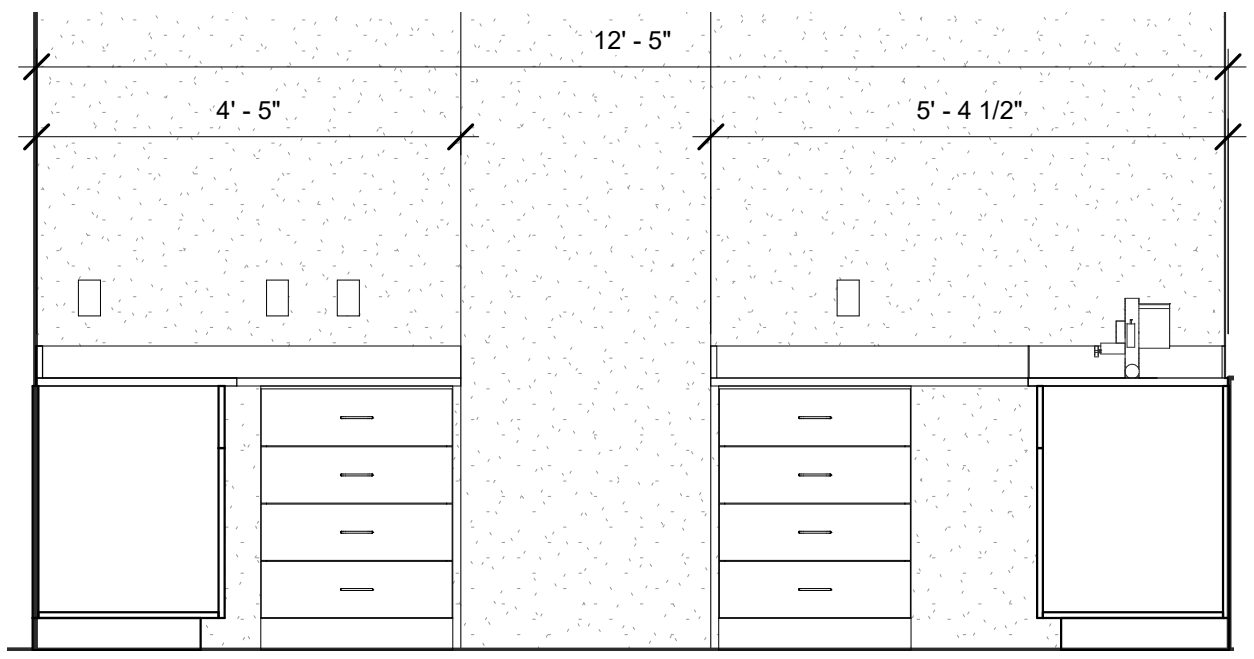
③ A402B - Model Making, West 1/2" = 1'-0"
