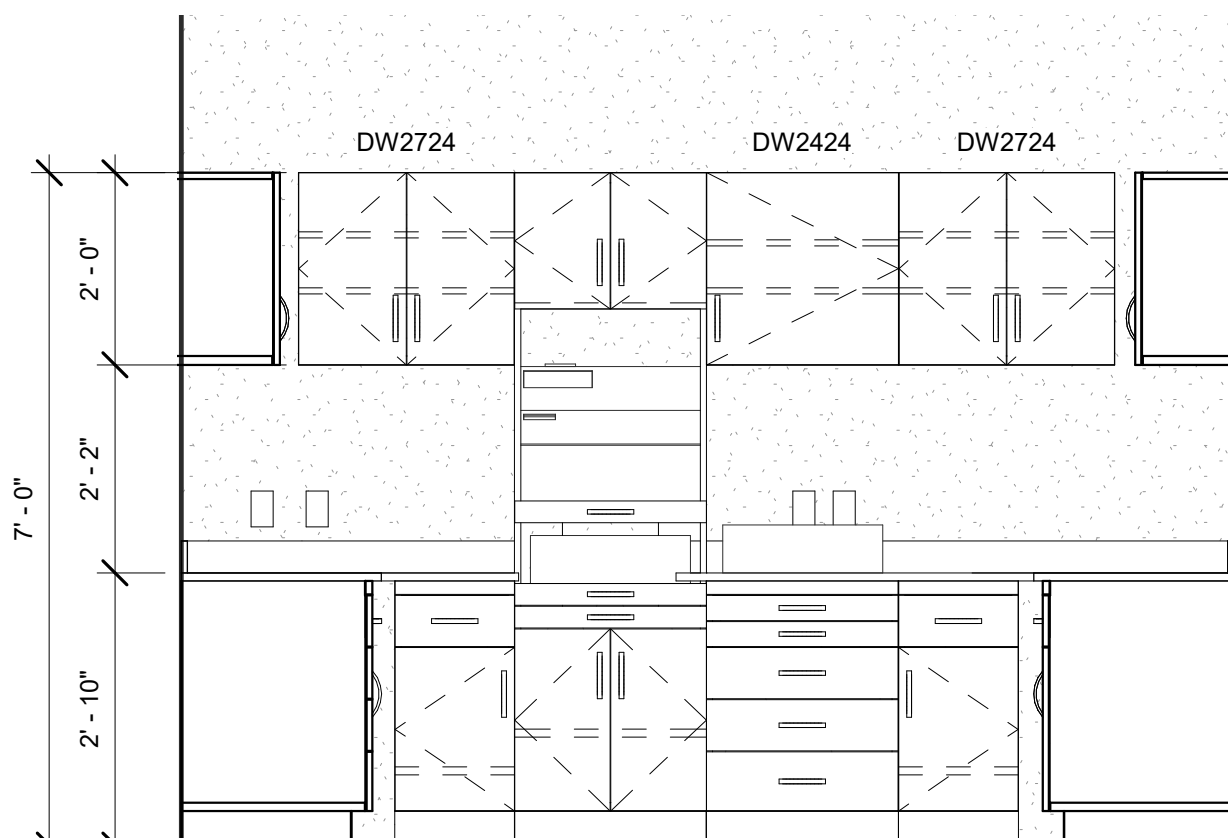
⑪ A402M - Steralization, South 1/2" = 1'-0"
