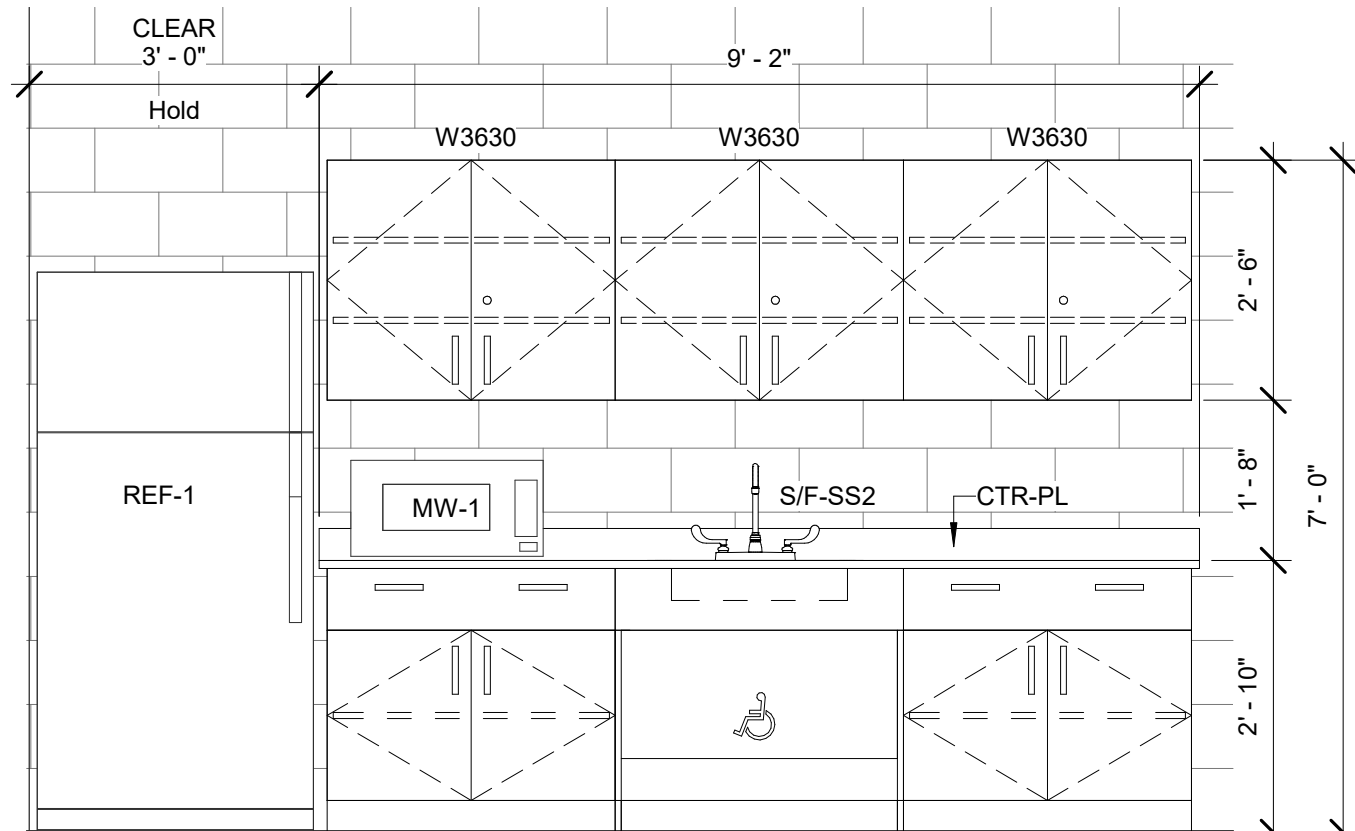
19 C020 - Cust Workshop 1/2" = 1'-0"
