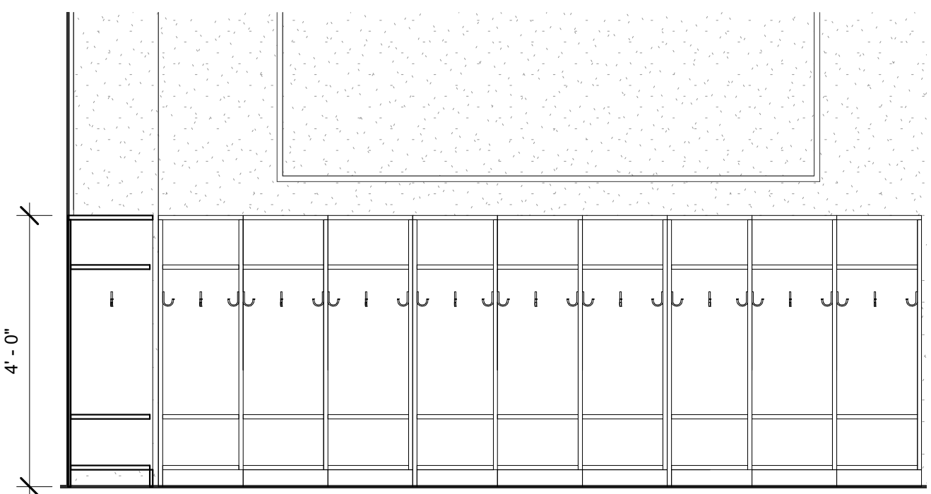
17 C106A - CUBBIES, South 1/2" = 1'-0"
