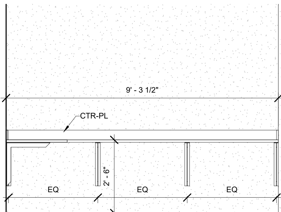
4 B201E- Drafting and Design- Office- West 1/2" = 1'-0"
