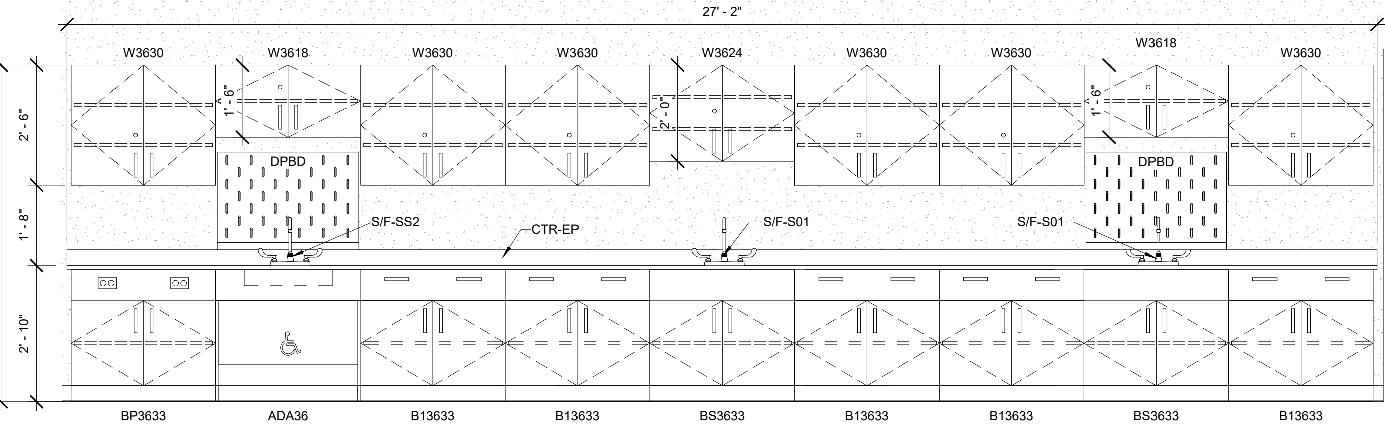
4 Science Lab - Typical for North & South 1/2" = 1'-0"
