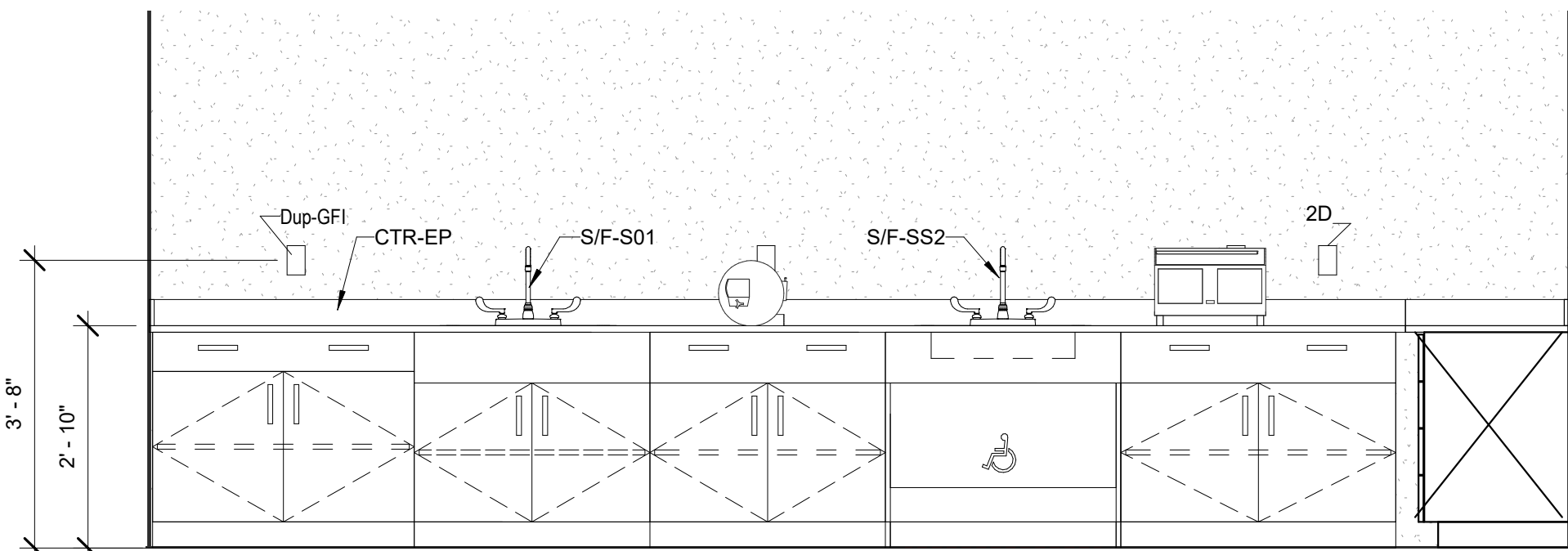
④ A402B - Model Making, South 1/2" = 1'-0"
