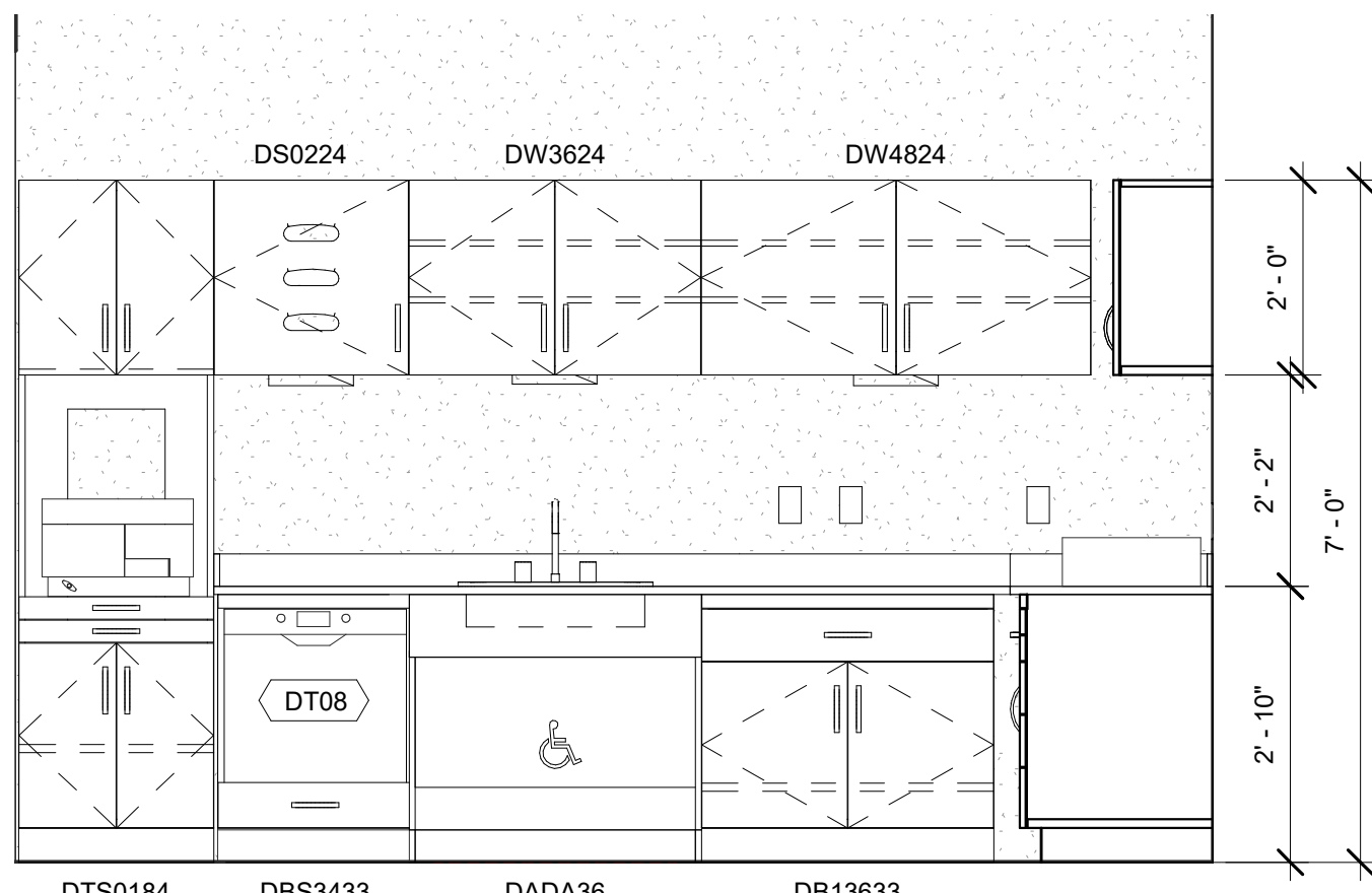
⑧ A402D - Steralization, East 1/2" = 1'-0"
