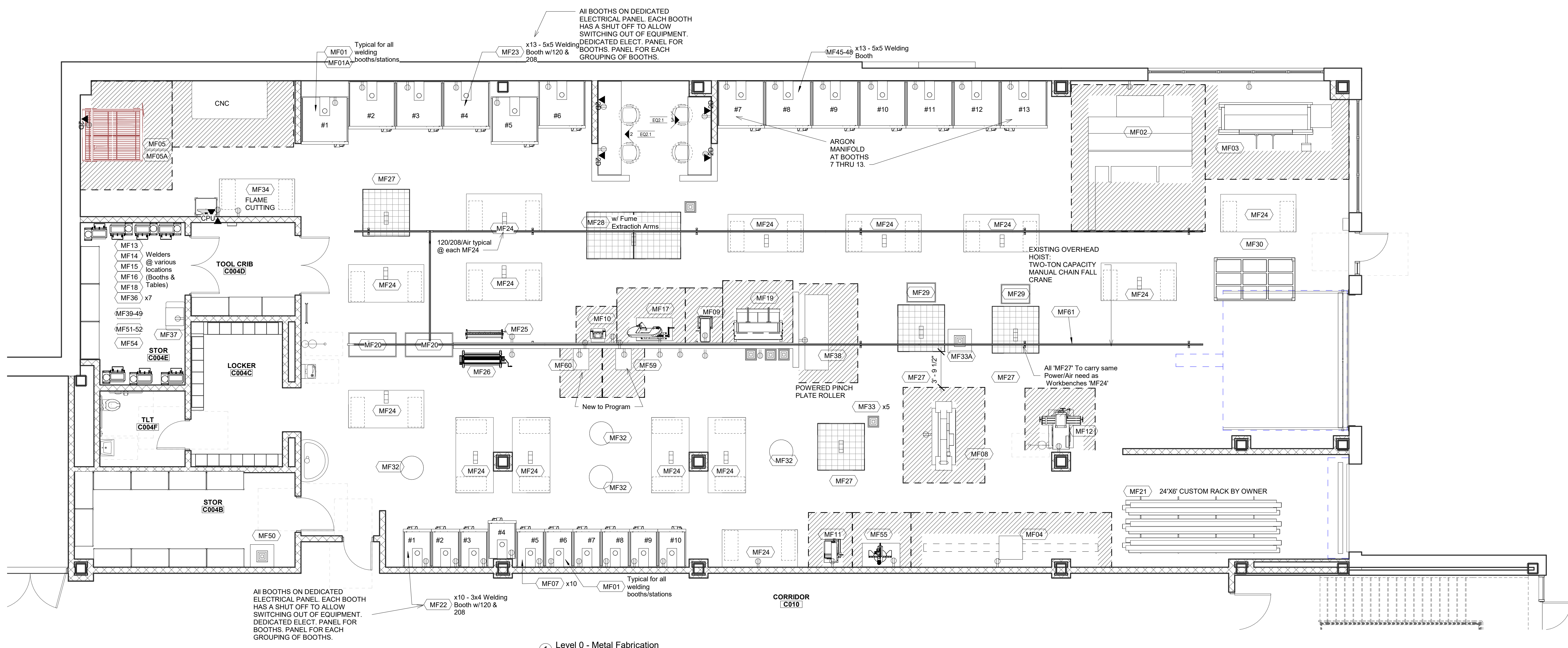
1 Level 0 - Metal Fabrication 3/16" = 1'-0"
