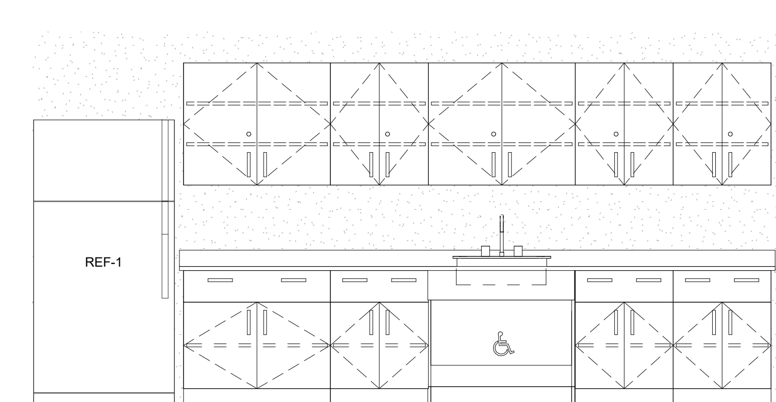
16 A111 - Staff Lunch, East 1/2" = 1'-0"
