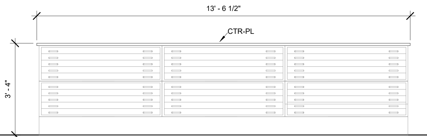
4 A206 - Design Visual Comm, Flat File Counter 1/2" = 1'-0"
