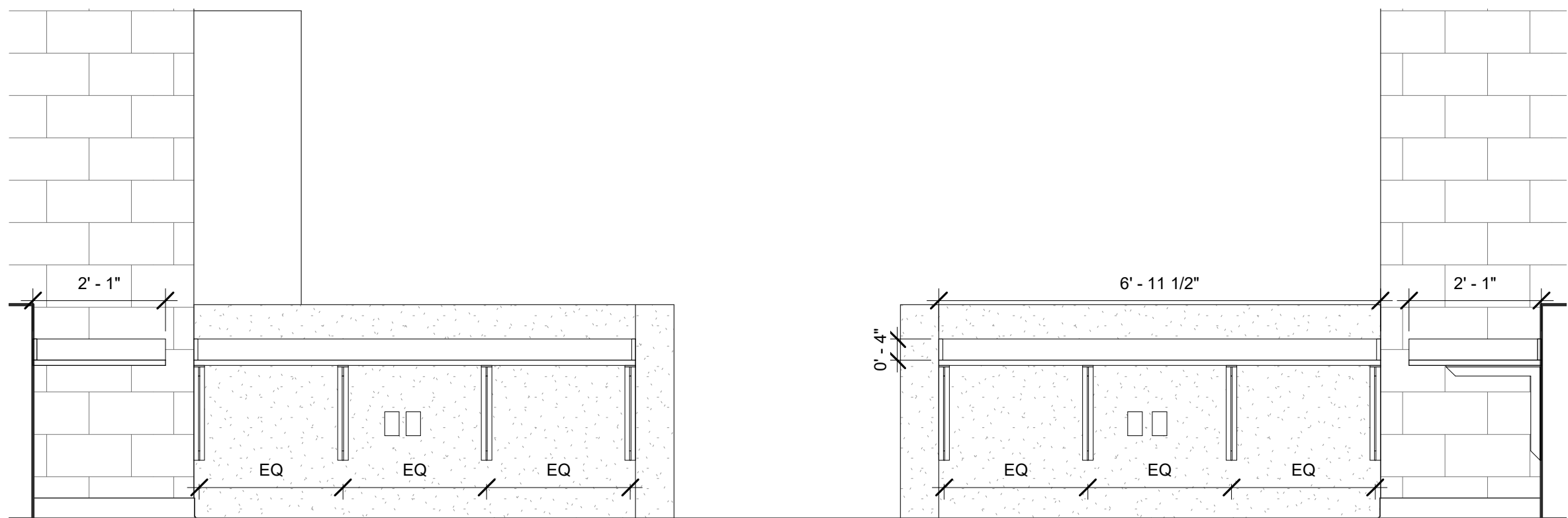
2 B103-Hvac- Office- West 1/2" = 1'-0"
