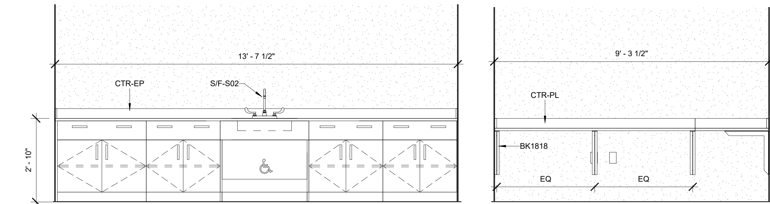
5 A303A - BioTech - Prep 1/2" = 1'-0"
