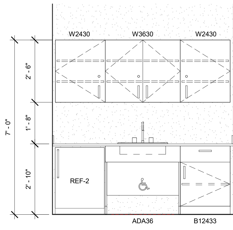
2 D109 - Nurse, Exam, South 1/2" = 1'-0"
