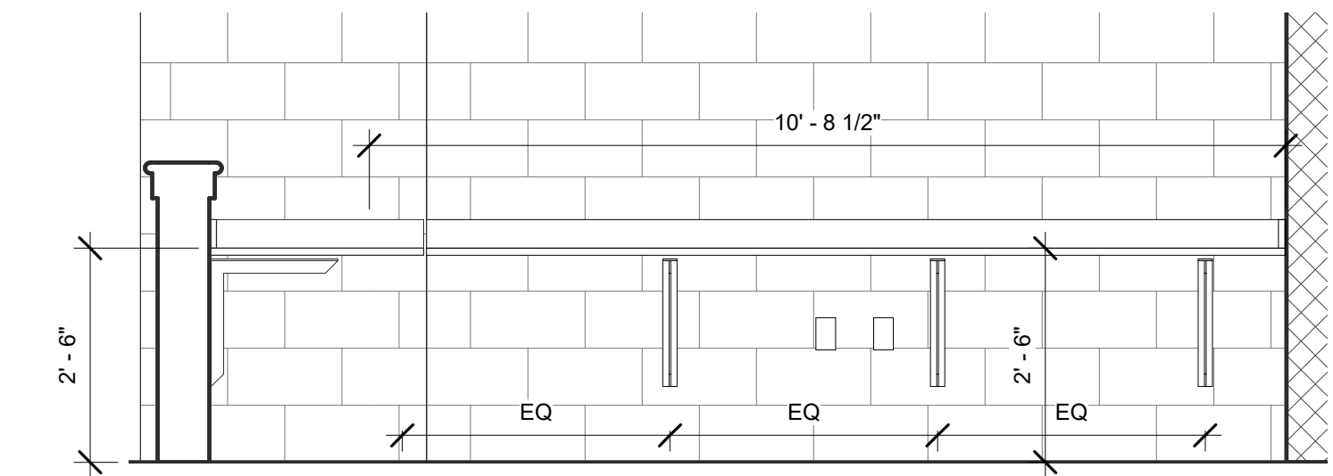
3 A141F - Carpentry - Staff Office - East 1/2" = 1'-0"
