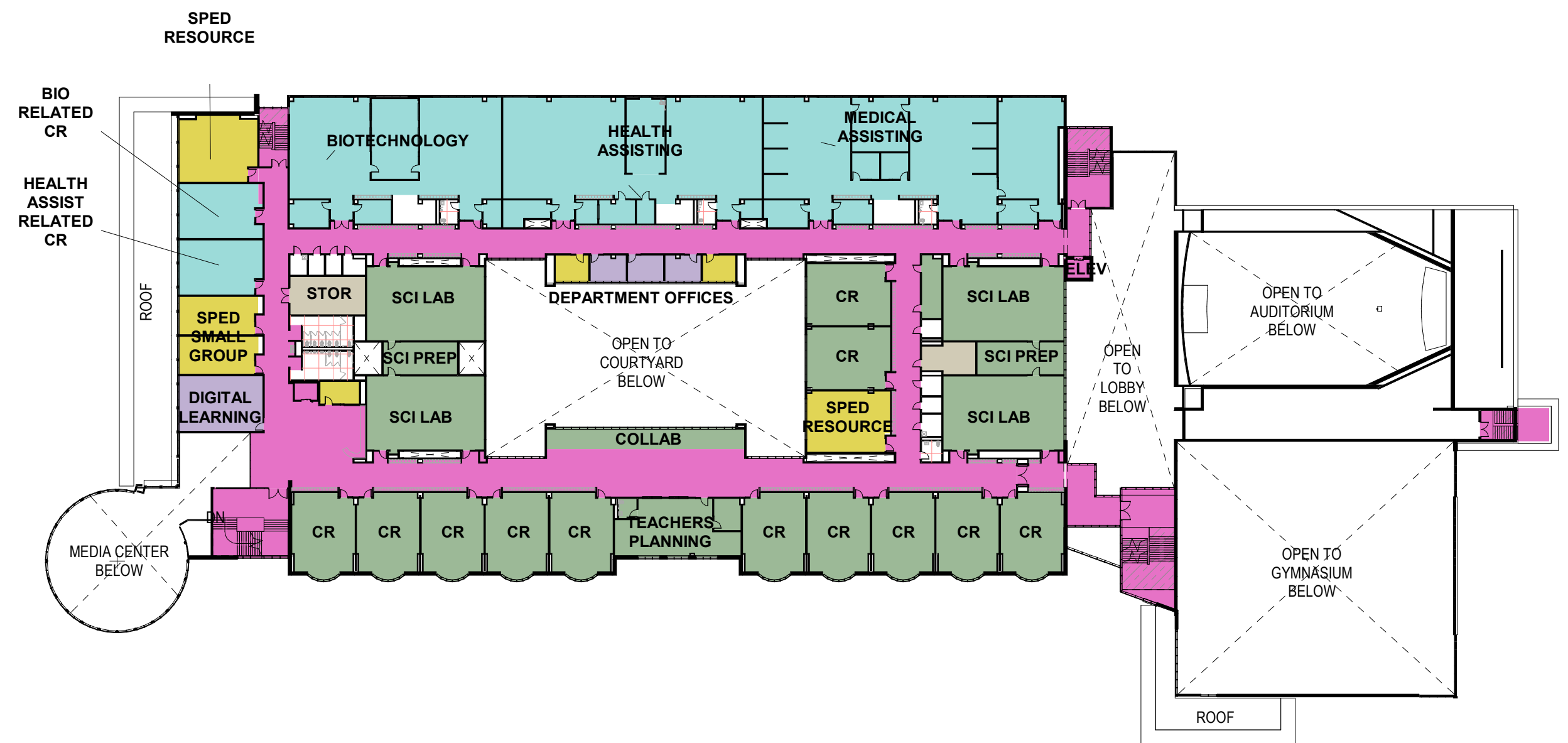
1 Third Floor Plan 1" = 50'-0"
